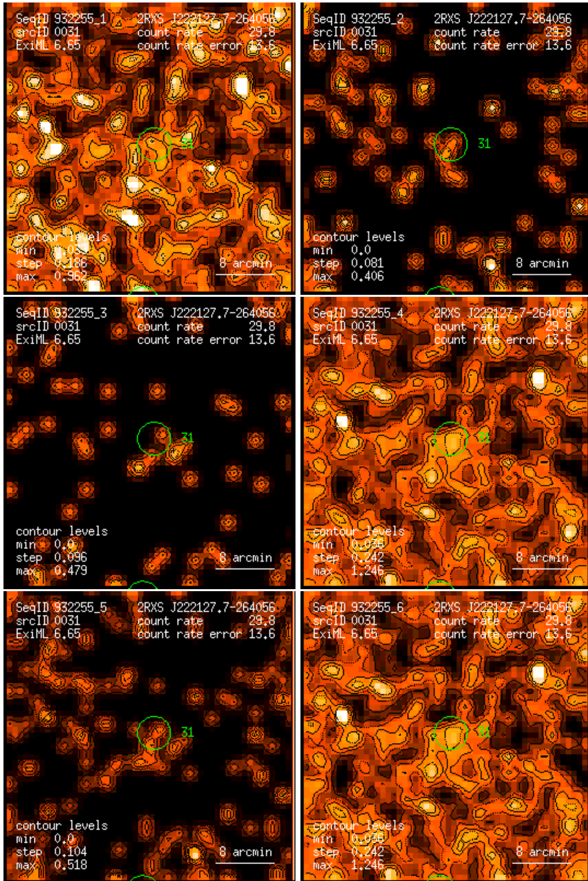
Figure 31: RASS 932255: detection 0031: band rate images, Gaussian filter: (1) PSPC channels 11 – 41, (2) 52 – 90, (3) 91 – 201, (4) 11 – 235, (5) 52 – 201, (6) 11 – 201. Broad band rates in counts/ks. Band rate contour levels in counts/ks/arcmin 2 .
