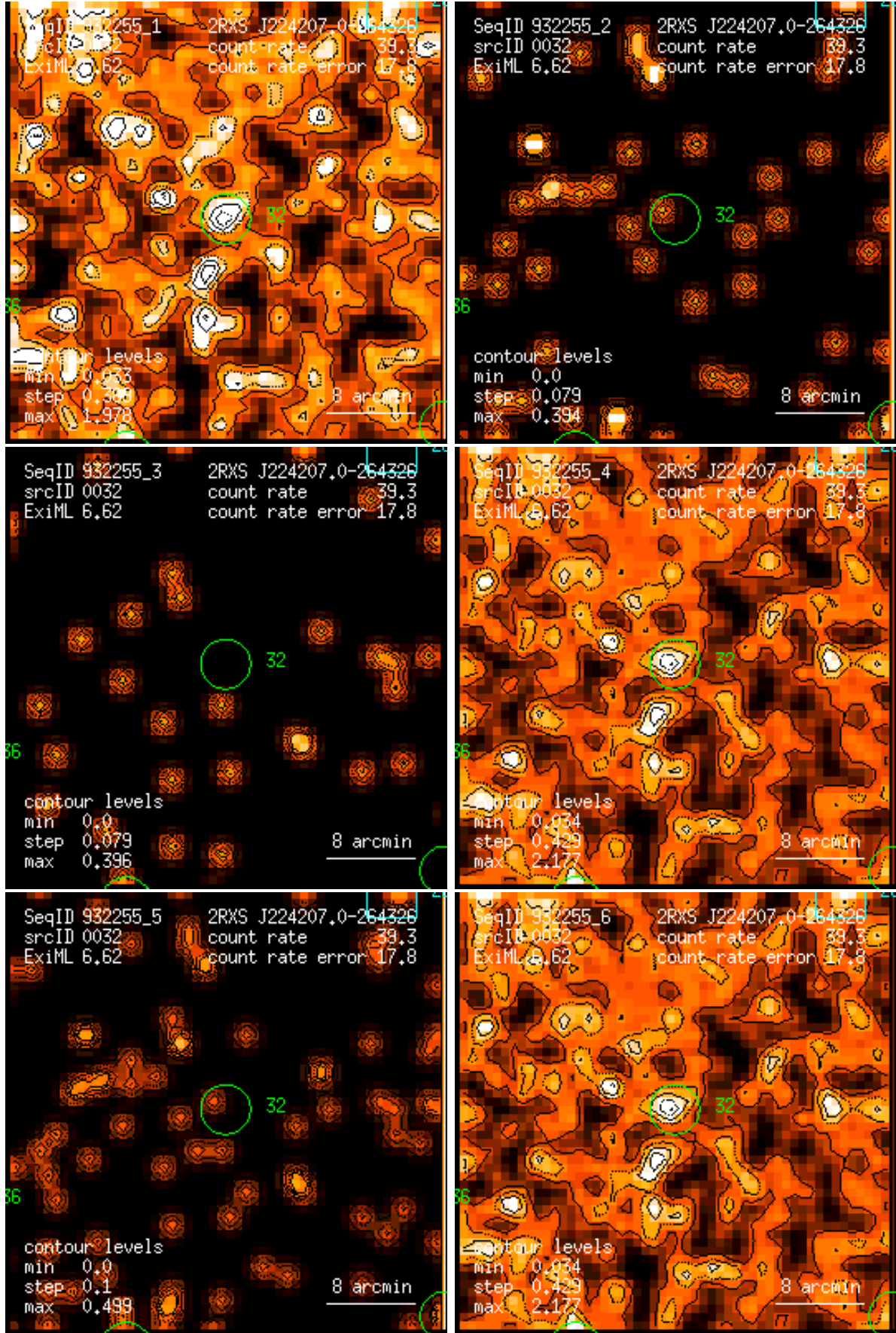
Figure 32: RASS 932255: detection 0032: band rate images, Gaussian filter: (1) PSPC channels 11 – 41, (2) 52 – 90, (3) 91 – 201, (4) 11 – 235, (5) 52 – 201, (6) 11 – 201. Broad band rates in counts/ks. Band rate contour levels in counts/ks/arcmin 2 .
