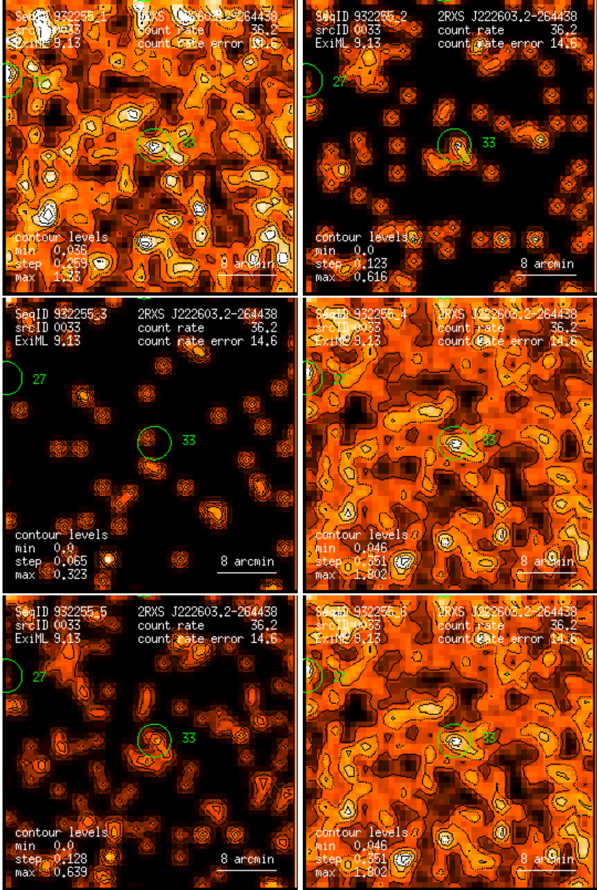
Figure 33: RASS 932255: detection 0033: band rate images, Gaussian filter: (1) PSPC channels 11 – 41, (2) 52 – 90, (3) 91 – 201, (4) 11 – 235, (5) 52 – 201, (6) 11 – 201. Broad band rates in counts/ks. Band rate contour levels in counts/ks/arcmin 2 .
