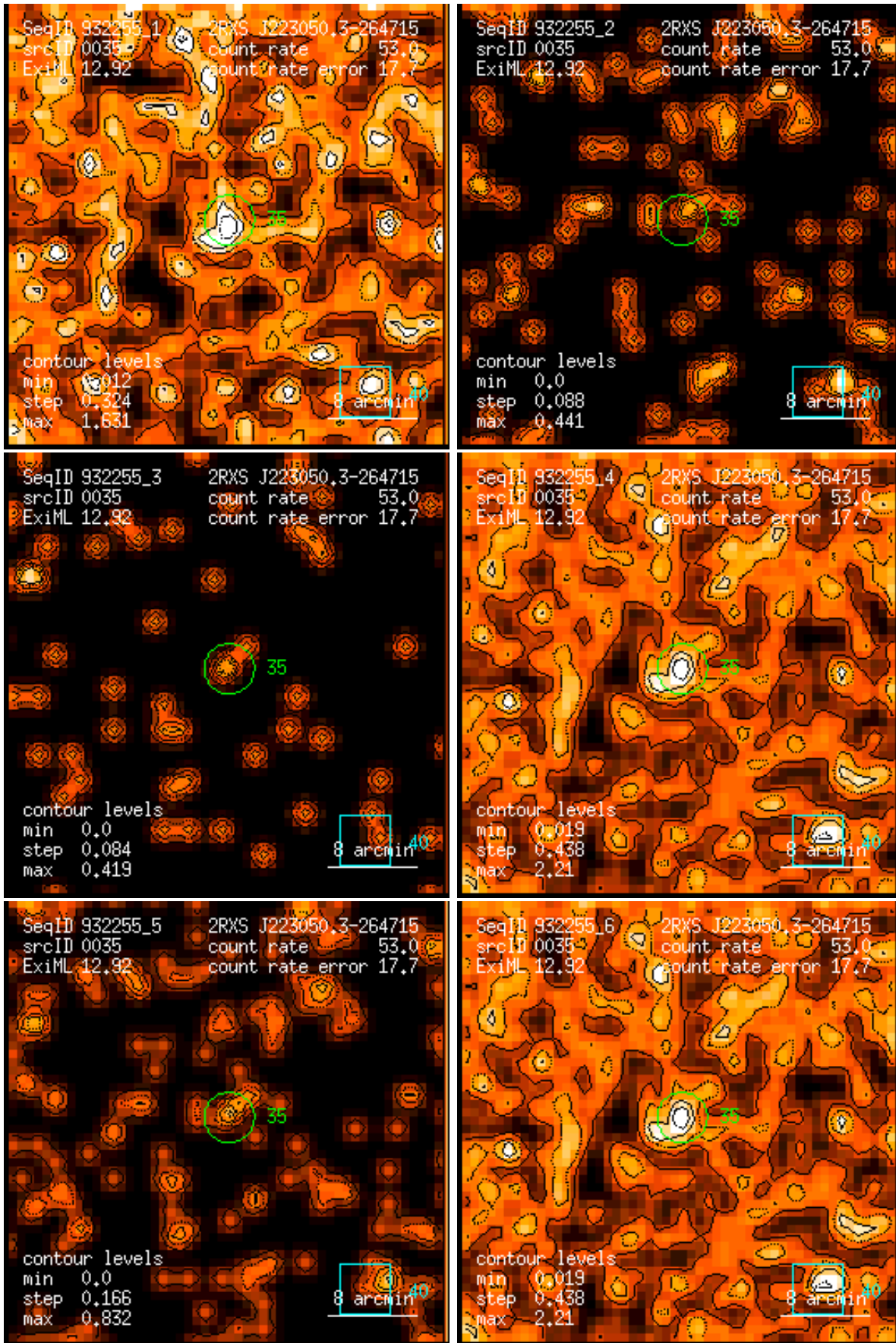
Figure 35: RASS 932255: detection 0035: band rate images, Gaussian filter: (1) PSPC channels 11 – 41, (2) 52 – 90, (3) 91 – 201, (4) 11 – 235, (5) 52 – 201, (6) 11 – 201. Broad band rates in counts/ks. Band rate contour levels in counts/ks/arcmin 2 .
