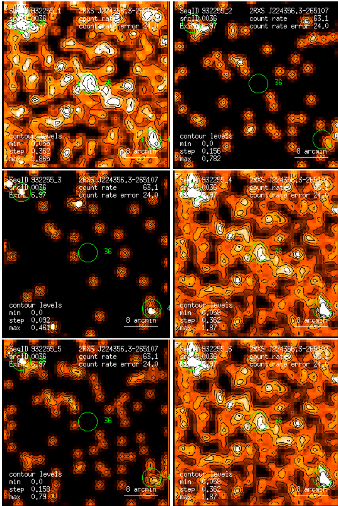
Figure 36: RASS 932255: detection 0036: band rate images, Gaussian filter: (1) PSPC channels 11 – 41, (2) 52 – 90, (3) 91 – 201, (4) 11 – 235, (5) 52 – 201, (6) 11 – 201. Broad band rates in counts/ks. Band rate contour levels in counts/ks/arcmin 2 .
