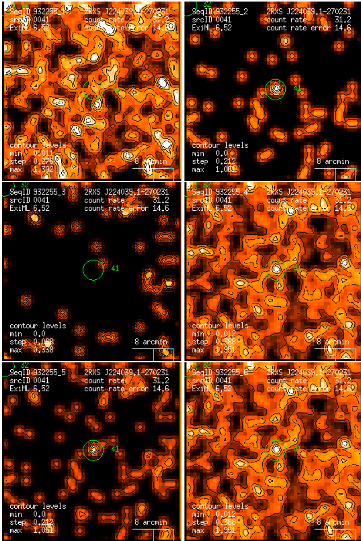
Figure 41: RASS 932255: detection 0041: band rate images, Gaussian filter: (1) PSPC channels 11 – 41, (2) 52 – 90, (3) 91 – 201, (4) 11 – 235, (5) 52 – 201, (6) 11 – 201. Broad band rates in counts/ks. Band rate contour levels in counts/ks/arcmin 2 .
