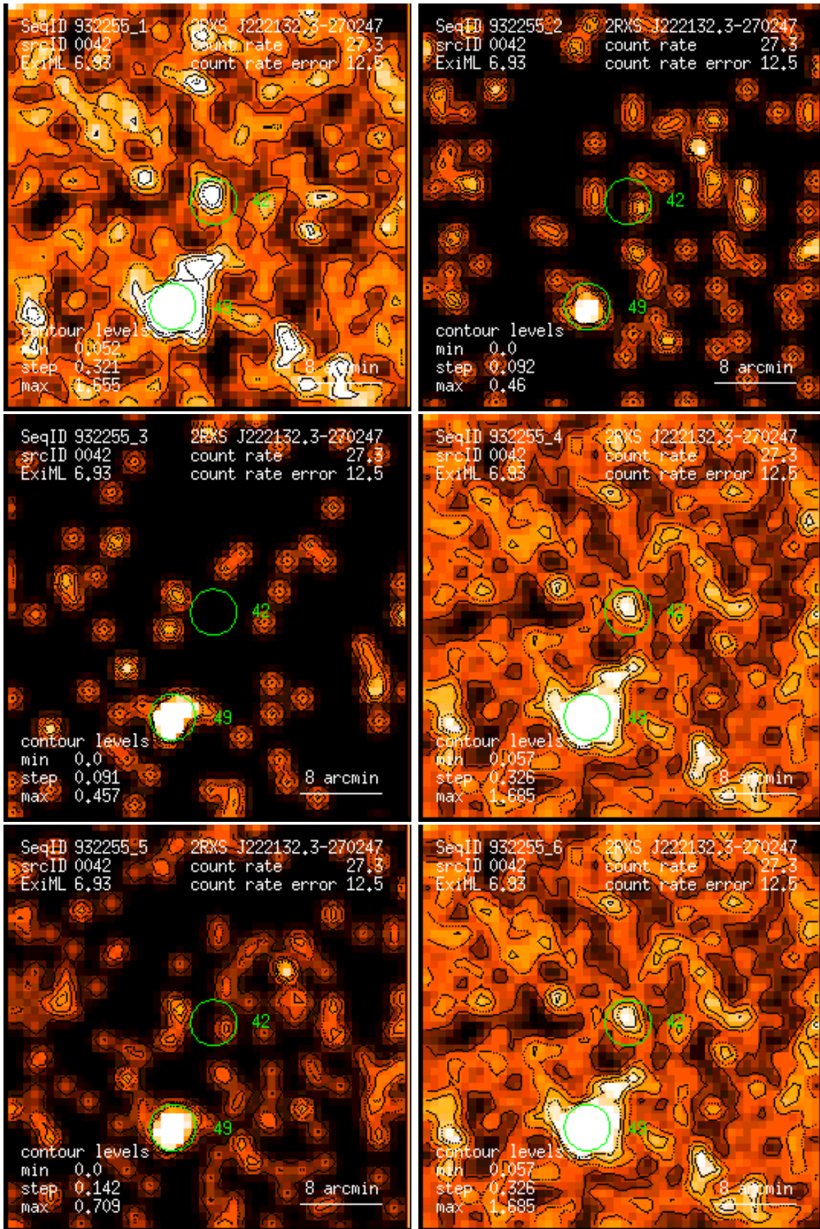
Figure 42: RASS 932255: detection 0042: band rate images, Gaussian filter: (1) PSPC channels 11 – 41, (2) 52 – 90, (3) 91 – 201, (4) 11 – 235, (5) 52 – 201, (6) 11 – 201. Broad band rates in counts/ks. Band rate contour levels in counts/ks/arcmin 2 .
