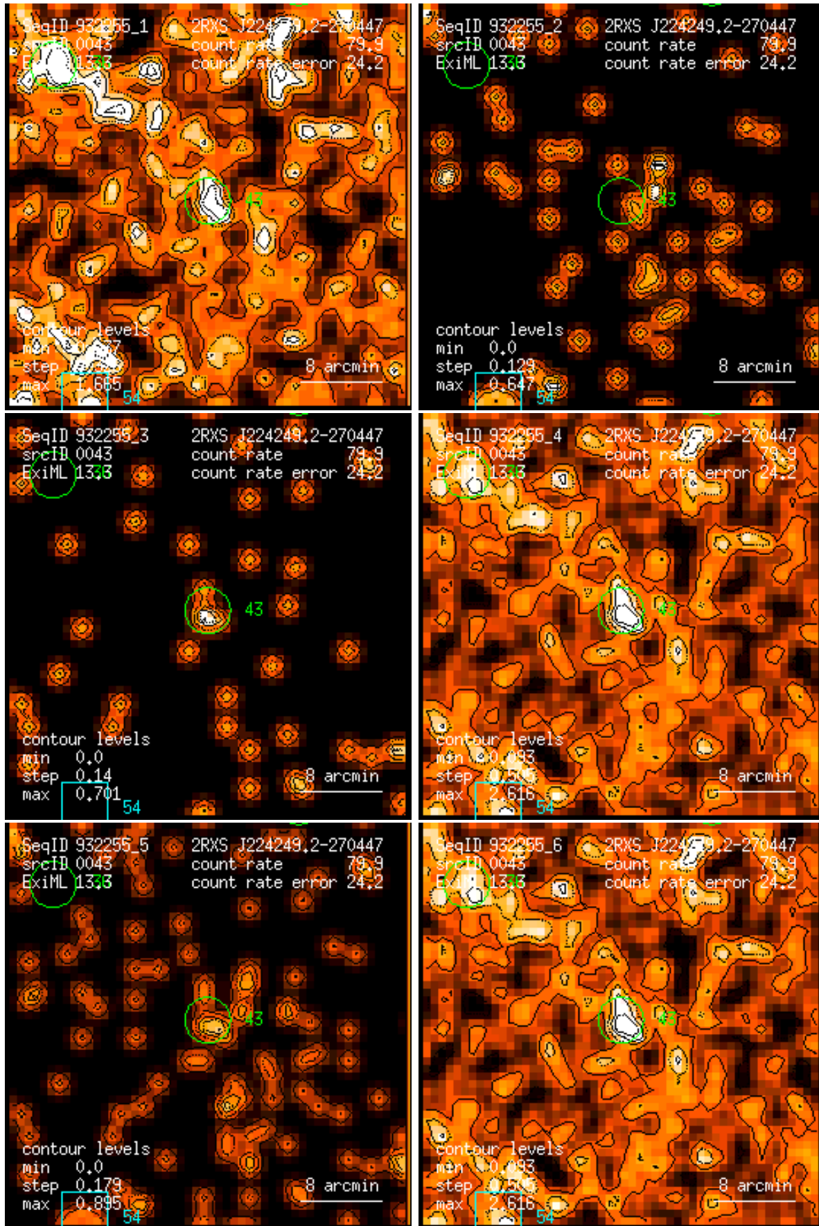
Figure 43: RASS 932255: detection 0043: band rate images, Gaussian filter: (1) PSPC channels 11 – 41, (2) 52 – 90, (3) 91 – 201, (4) 11 – 235, (5) 52 – 201, (6) 11 – 201. Broad band rates in counts/ks. Band rate contour levels in counts/ks/arcmin 2 .
