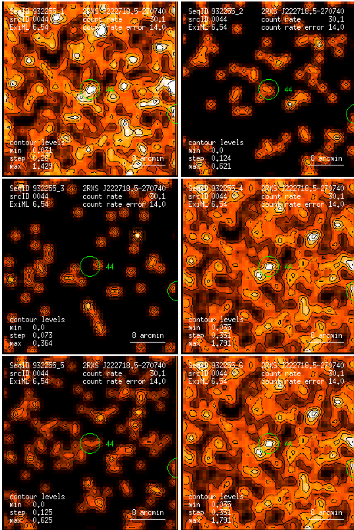
Figure 44: RASS 932255: detection 0044: band rate images, Gaussian filter: (1) PSPC channels 11 – 41, (2) 52 – 90, (3) 91 – 201, (4) 11 – 235, (5) 52 – 201, (6) 11 – 201. Broad band rates in counts/ks. Band rate contour levels in counts/ks/arcmin 2 .
