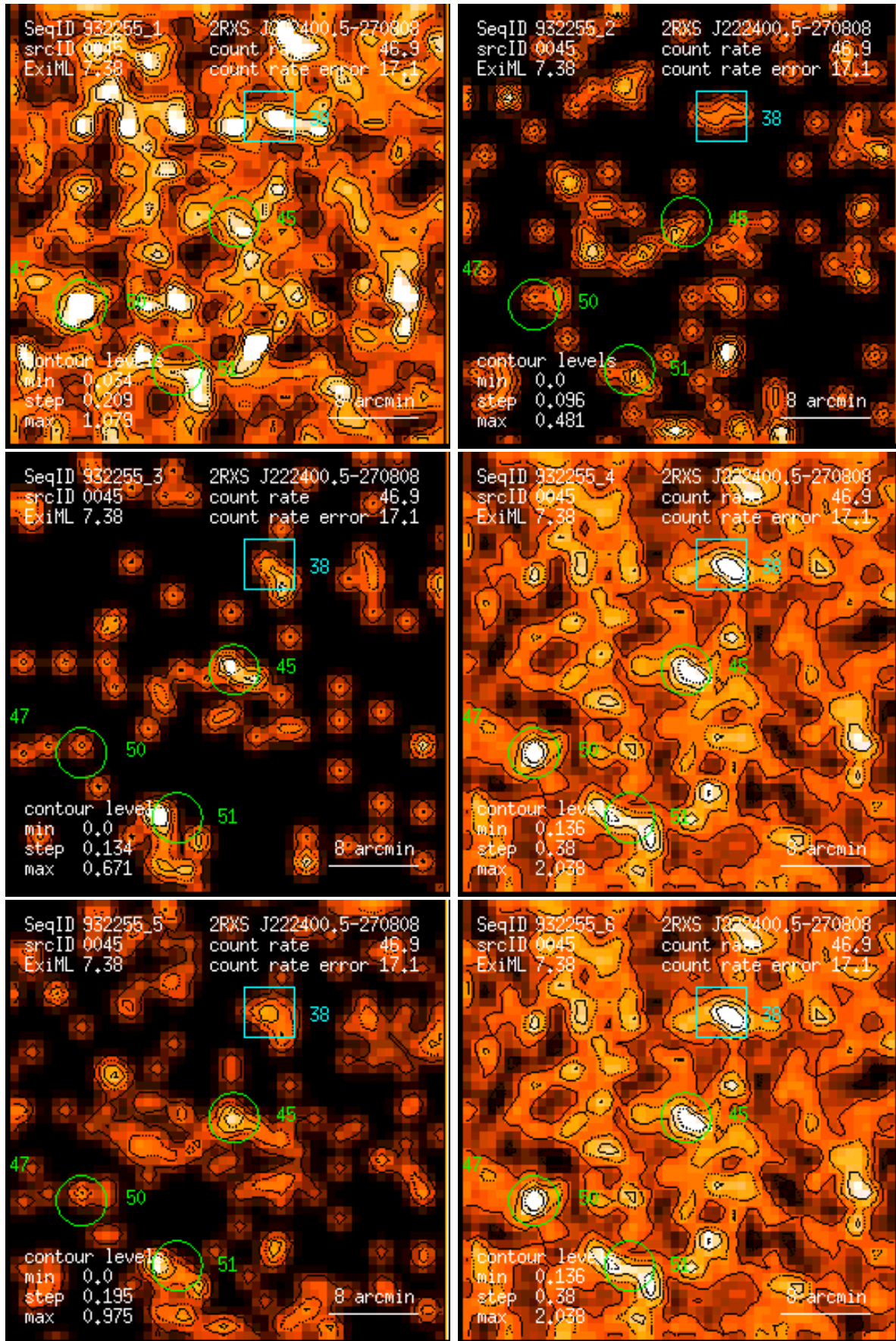
Figure 45: RASS 932255: detection 0045: band rate images, Gaussian filter: (1) PSPC channels 11 – 41, (2) 52 – 90, (3) 91 – 201, (4) 11 – 235, (5) 52 – 201, (6) 11 – 201. Broad band rates in counts/ks. Band rate contour levels in counts/ks/arcmin 2 .
