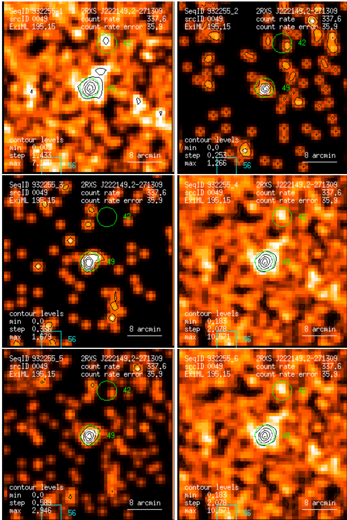
Figure 49: RASS 932255: detection 0049: band rate images, Gaussian filter: (1) PSPC channels 11 – 41, (2) 52 – 90, (3) 91 – 201, (4) 11 – 235, (5) 52 – 201, (6) 11 – 201. Broad band rates in counts/ks. Band rate contour levels in counts/ks/arcmin 2 .
