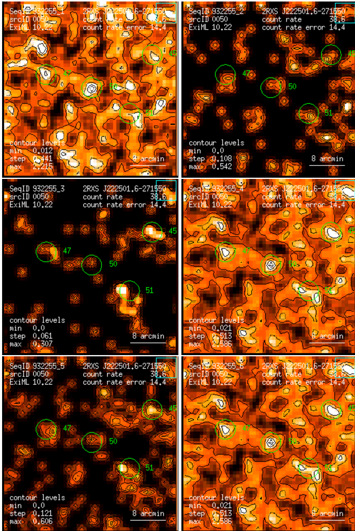
Figure 50: RASS 932255: detection 0050: band rate images, Gaussian filter: (1) PSPC channels 11 – 41, (2) 52 – 90, (3) 91 – 201, (4) 11 – 235, (5) 52 – 201, (6) 11 – 201. Broad band rates in counts/ks. Band rate contour levels in counts/ks/arcmin 2 .
