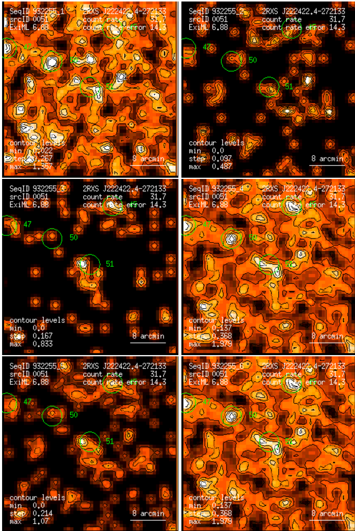
Figure 51: RASS 932255: detection 0051: band rate images, Gaussian filter: (1) PSPC channels 11 – 41, (2) 52 – 90, (3) 91 – 201, (4) 11 – 235, (5) 52 – 201, (6) 11 – 201. Broad band rates in counts/ks. Band rate contour levels in counts/ks/arcmin 2 .
