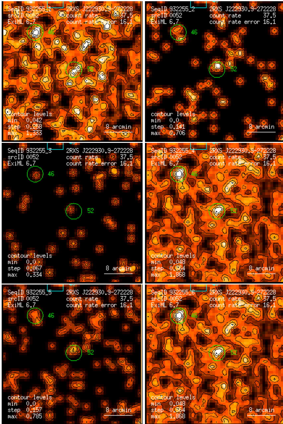
Figure 52: RASS 932255: detection 0052: band rate images, Gaussian filter: (1) PSPC channels 11 – 41, (2) 52 – 90, (3) 91 – 201, (4) 11 – 235, (5) 52 – 201, (6) 11 – 201. Broad band rates in counts/ks. Band rate contour levels in counts/ks/arcmin 2 .
