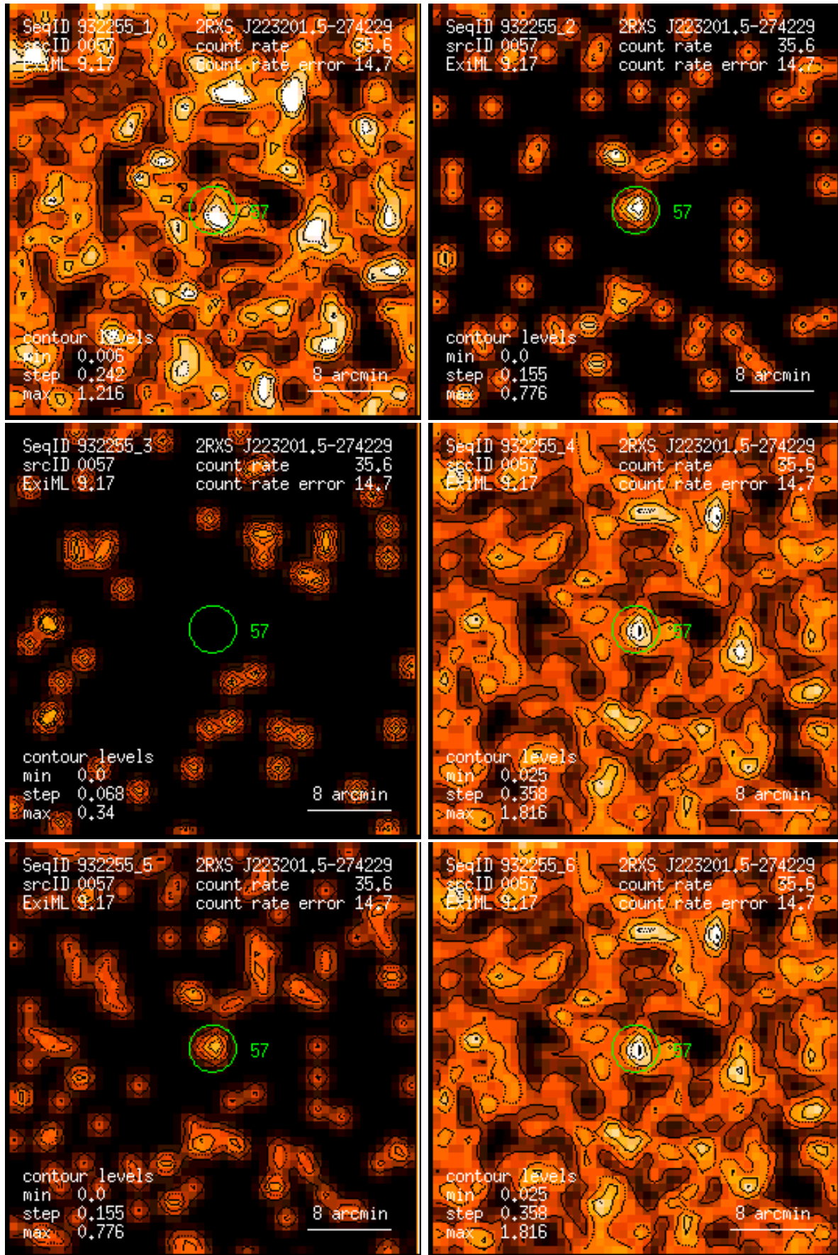
Figure 57: RASS 932255: detection 0057: band rate images, Gaussian filter: (1) PSPC channels 11 – 41, (2) 52 – 90, (3) 91 – 201, (4) 11 – 235, (5) 52 – 201, (6) 11 – 201. Broad band rates in counts/ks. Band rate contour levels in counts/ks/arcmin 2 .
