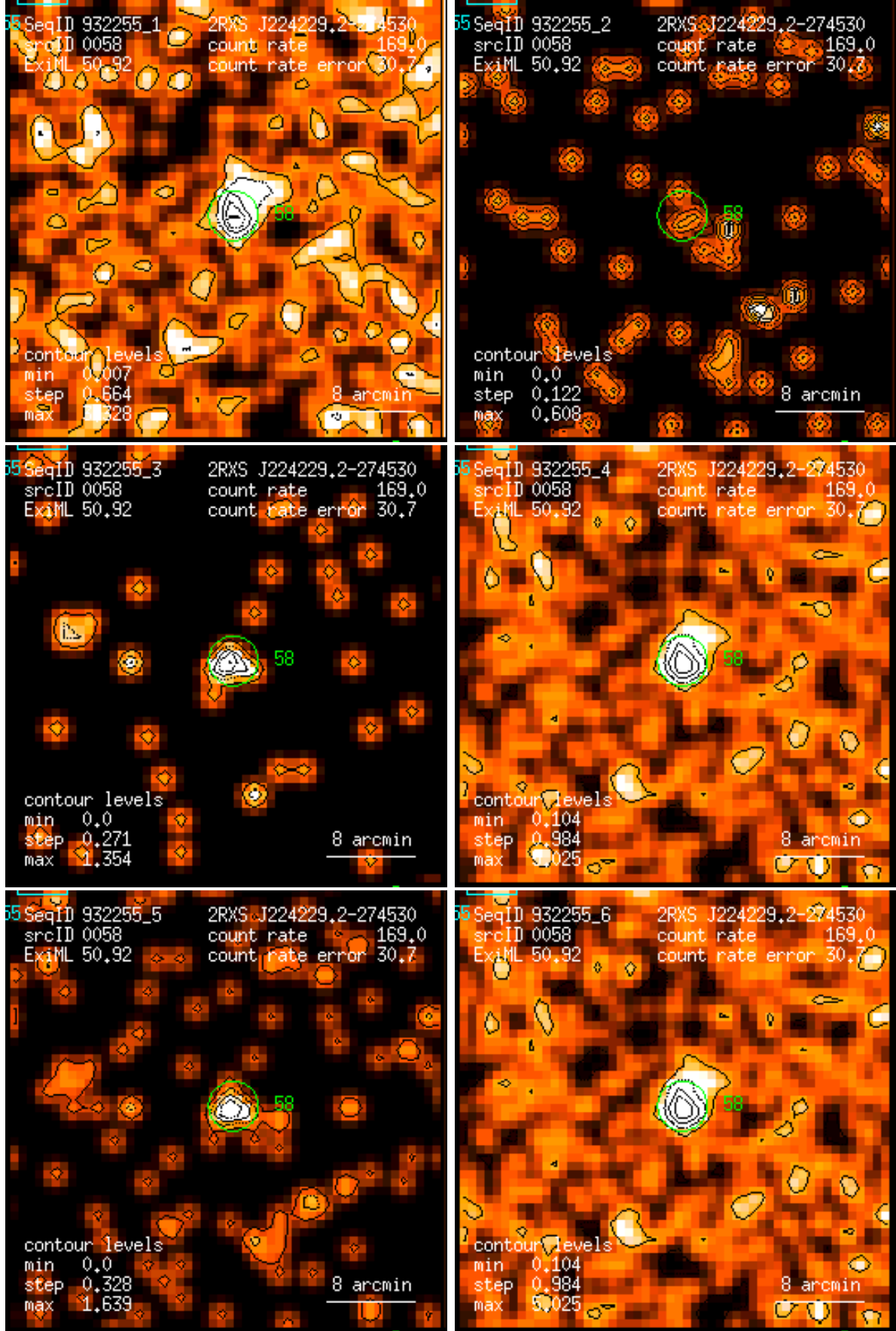
Figure 58: RASS 932255: detection 0058: band rate images, Gaussian filter: (1) PSPC channels 11 – 41, (2) 52 – 90, (3) 91 – 201, (4) 11 – 235, (5) 52 – 201, (6) 11 – 201. Broad band rates in counts/ks. Band rate contour levels in counts/ks/arcmin 2 .
