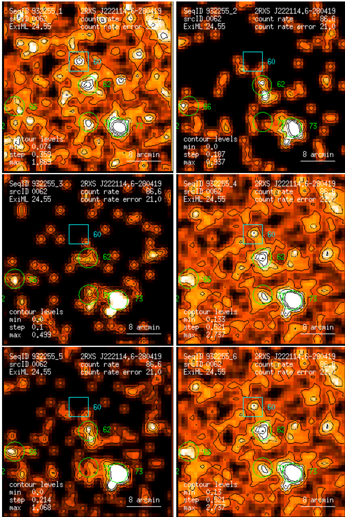
Figure 62: RASS 932255: detection 0062: band rate images, Gaussian filter: (1) PSPC channels 11 – 41, (2) 52 – 90, (3) 91 – 201, (4) 11 – 235, (5) 52 – 201, (6) 11 – 201. Broad band rates in counts/ks. Band rate contour levels in counts/ks/arcmin 2 .
