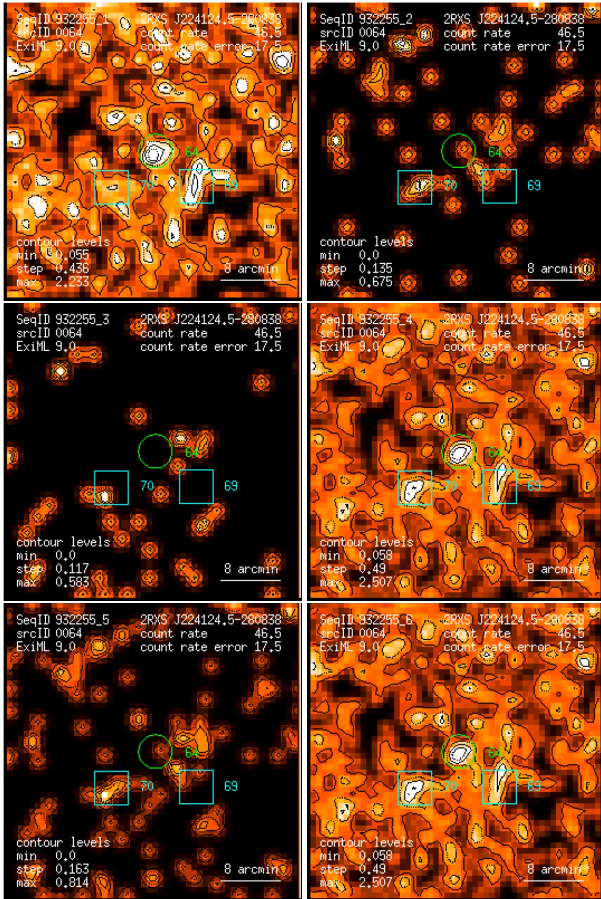
Figure 64: RASS 932255: detection 0064: band rate images, Gaussian filter: (1) PSPC channels 11 – 41, (2) 52 – 90, (3) 91 – 201, (4) 11 – 235, (5) 52 – 201, (6) 11 – 201. Broad band rates in counts/ks. Band rate contour levels in counts/ks/arcmin 2 .
