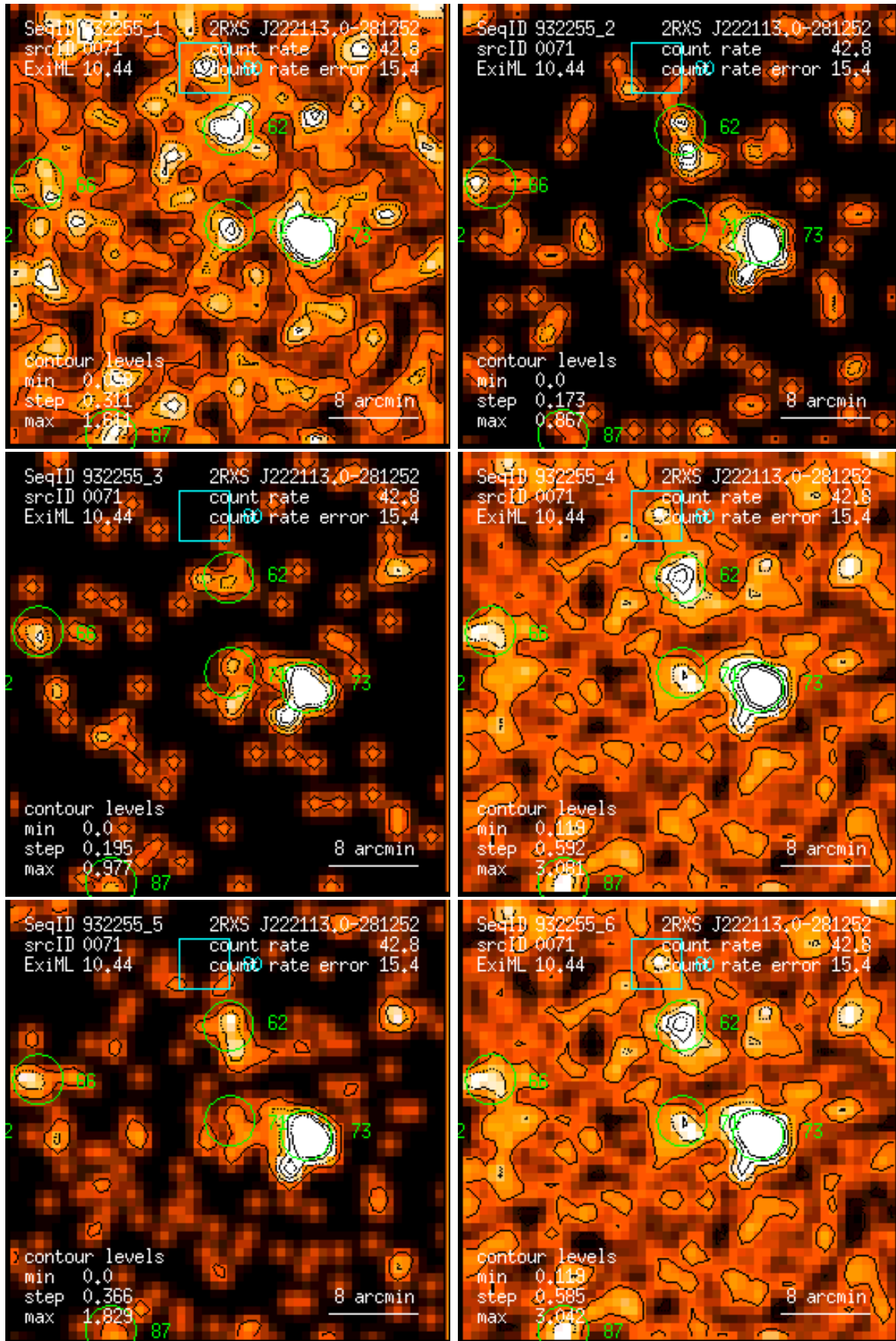
Figure 71: RASS 932255: detection 0071: band rate images, Gaussian filter: (1) PSPC channels 11 – 41, (2) 52 – 90, (3) 91 – 201, (4) 11 – 235, (5) 52 – 201, (6) 11 – 201. Broad band rates in counts/ks. Band rate contour levels in counts/ks/arcmin 2 .
