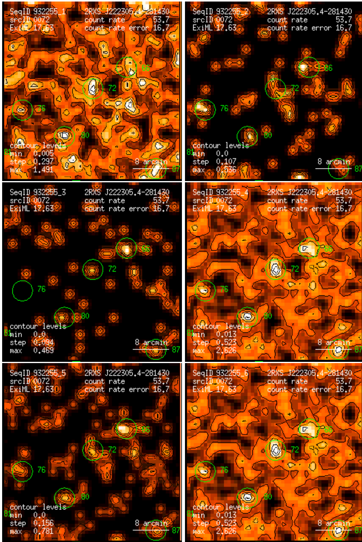
Figure 72: RASS 932255: detection 0072: band rate images, Gaussian filter: (1) PSPC channels 11 – 41, (2) 52 – 90, (3) 91 – 201, (4) 11 – 235, (5) 52 – 201, (6) 11 – 201. Broad band rates in counts/ks. Band rate contour levels in counts/ks/arcmin 2 .
