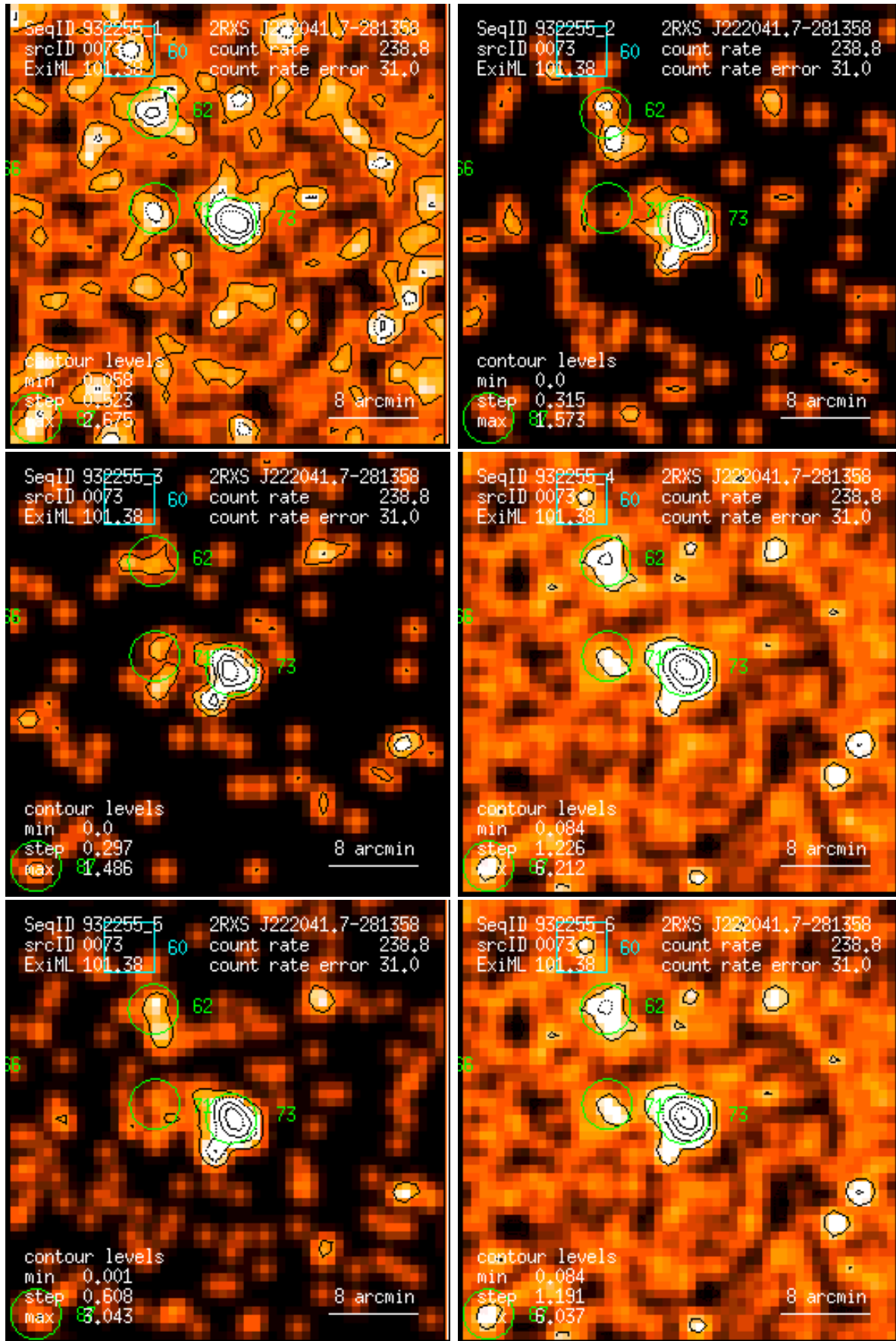
Figure 73: RASS 932255: detection 0073: band rate images, Gaussian filter: (1) PSPC channels 11 – 41, (2) 52 – 90, (3) 91 – 201, (4) 11 – 235, (5) 52 – 201, (6) 11 – 201. Broad band rates in counts/ks. Band rate contour levels in counts/ks/arcmin 2 .
