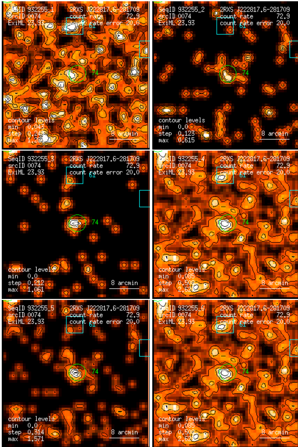
Figure 74: RASS 932255: detection 0074: band rate images, Gaussian filter: (1) PSPC channels 11 – 41, (2) 52 – 90, (3) 91 – 201, (4) 11 – 235, (5) 52 – 201, (6) 11 – 201. Broad band rates in counts/ks. Band rate contour levels in counts/ks/arcmin 2 .
