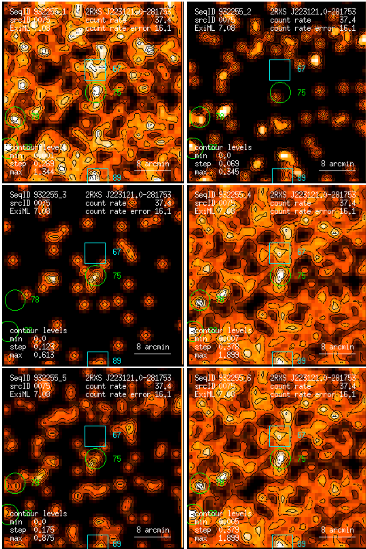
Figure 75: RASS 932255: detection 0075: band rate images, Gaussian filter: (1) PSPC channels 11 – 41, (2) 52 – 90, (3) 91 – 201, (4) 11 – 235, (5) 52 – 201, (6) 11 – 201. Broad band rates in counts/ks. Band rate contour levels in counts/ks/arcmin 2 .
