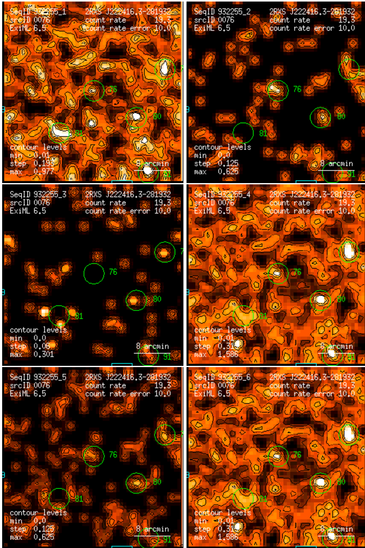
Figure 76: RASS 932255: detection 0076: band rate images, Gaussian filter: (1) PSPC channels 11 – 41, (2) 52 – 90, (3) 91 – 201, (4) 11 – 235, (5) 52 – 201, (6) 11 – 201. Broad band rates in counts/ks. Band rate contour levels in counts/ks/arcmin 2 .
