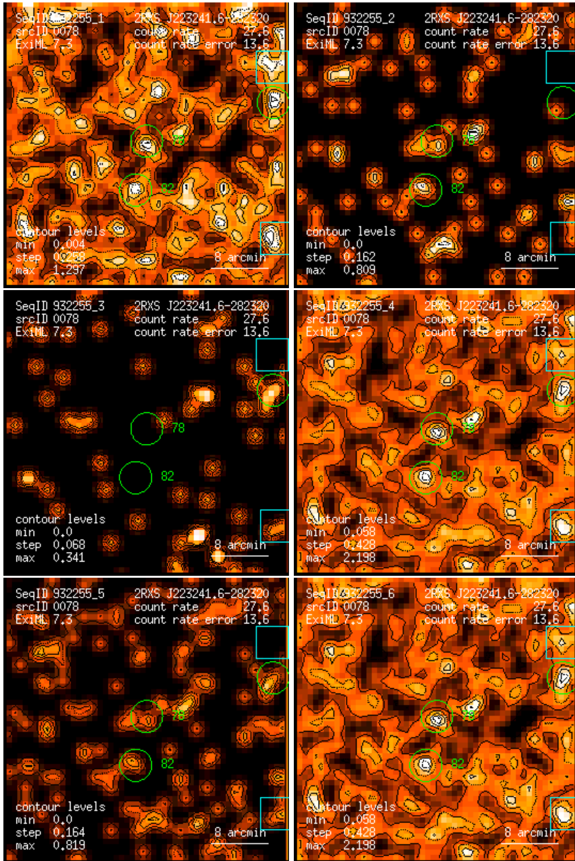
Figure 78: RASS 932255: detection 0078: band rate images, Gaussian filter: (1) PSPC channels 11 – 41, (2) 52 – 90, (3) 91 – 201, (4) 11 – 235, (5) 52 – 201, (6) 11 – 201. Broad band rates in counts/ks. Band rate contour levels in counts/ks/arcmin 2 .
