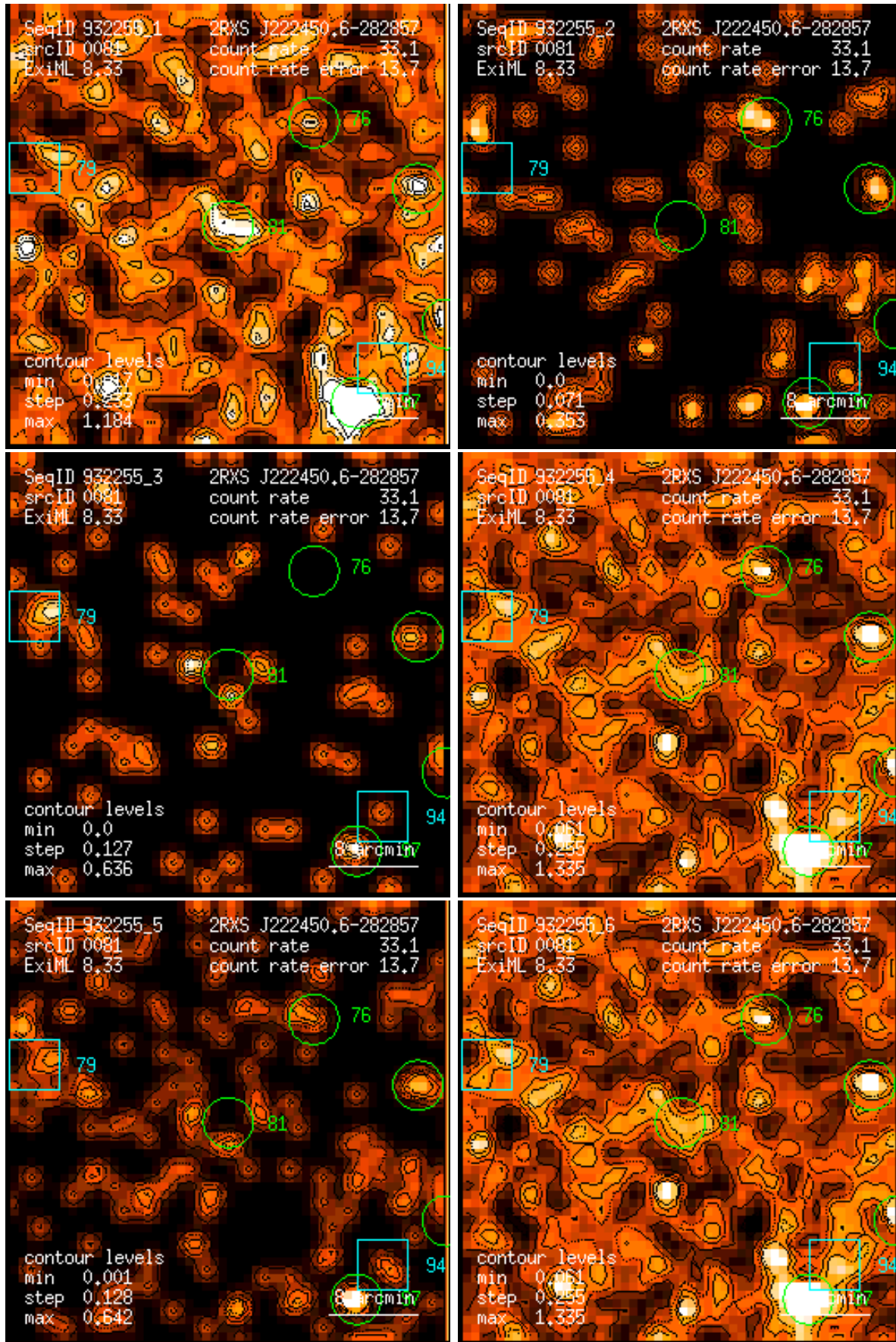
Figure 81: RASS 932255: detection 0081: band rate images, Gaussian filter: (1) PSPC channels 11 – 41, (2) 52 – 90, (3) 91 – 201, (4) 11 – 235, (5) 52 – 201, (6) 11 – 201. Broad band rates in counts/ks. Band rate contour levels in counts/ks/arcmin 2 .
