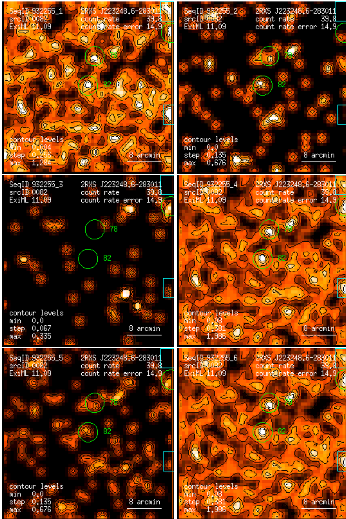
Figure 82: RASS 932255: detection 0082: band rate images, Gaussian filter: (1) PSPC channels 11 – 41, (2) 52 – 90, (3) 91 – 201, (4) 11 – 235, (5) 52 – 201, (6) 11 – 201. Broad band rates in counts/ks. Band rate contour levels in counts/ks/arcmin 2 .
