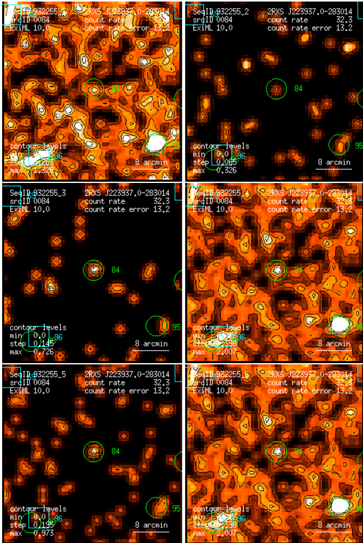
Figure 84: RASS 932255: detection 0084: band rate images, Gaussian filter: (1) PSPC channels 11 – 41, (2) 52 – 90, (3) 91 – 201, (4) 11 – 235, (5) 52 – 201, (6) 11 – 201. Broad band rates in counts/ks. Band rate contour levels in counts/ks/arcmin 2 .
