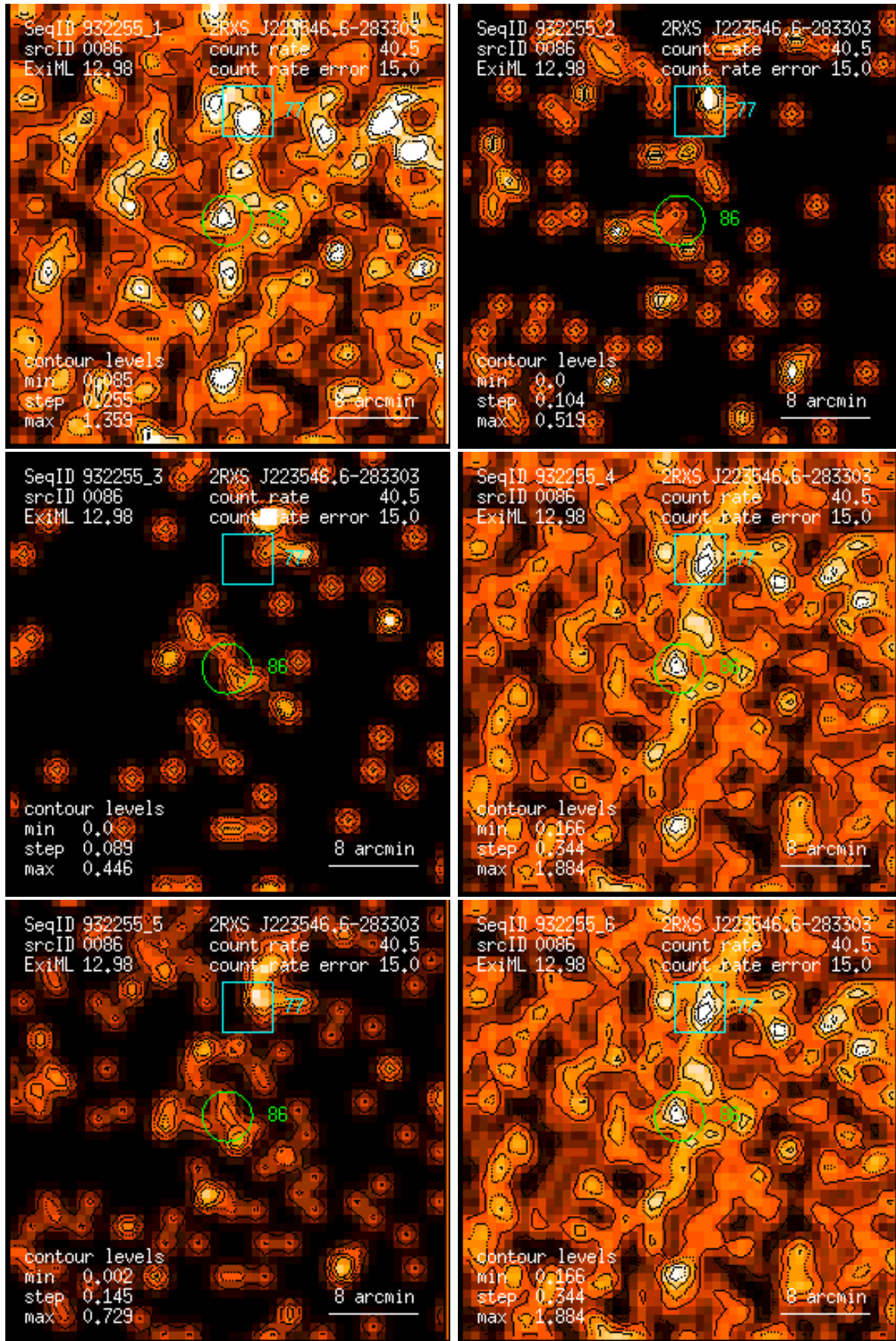
Figure 86: RASS 932255: detection 0086: band rate images, Gaussian filter: (1) PSPC channels 11 – 41, (2) 52 – 90, (3) 91 – 201, (4) 11 – 235, (5) 52 – 201, (6) 11 – 201. Broad band rates in counts/ks. Band rate contour levels in counts/ks/arcmin 2 .
