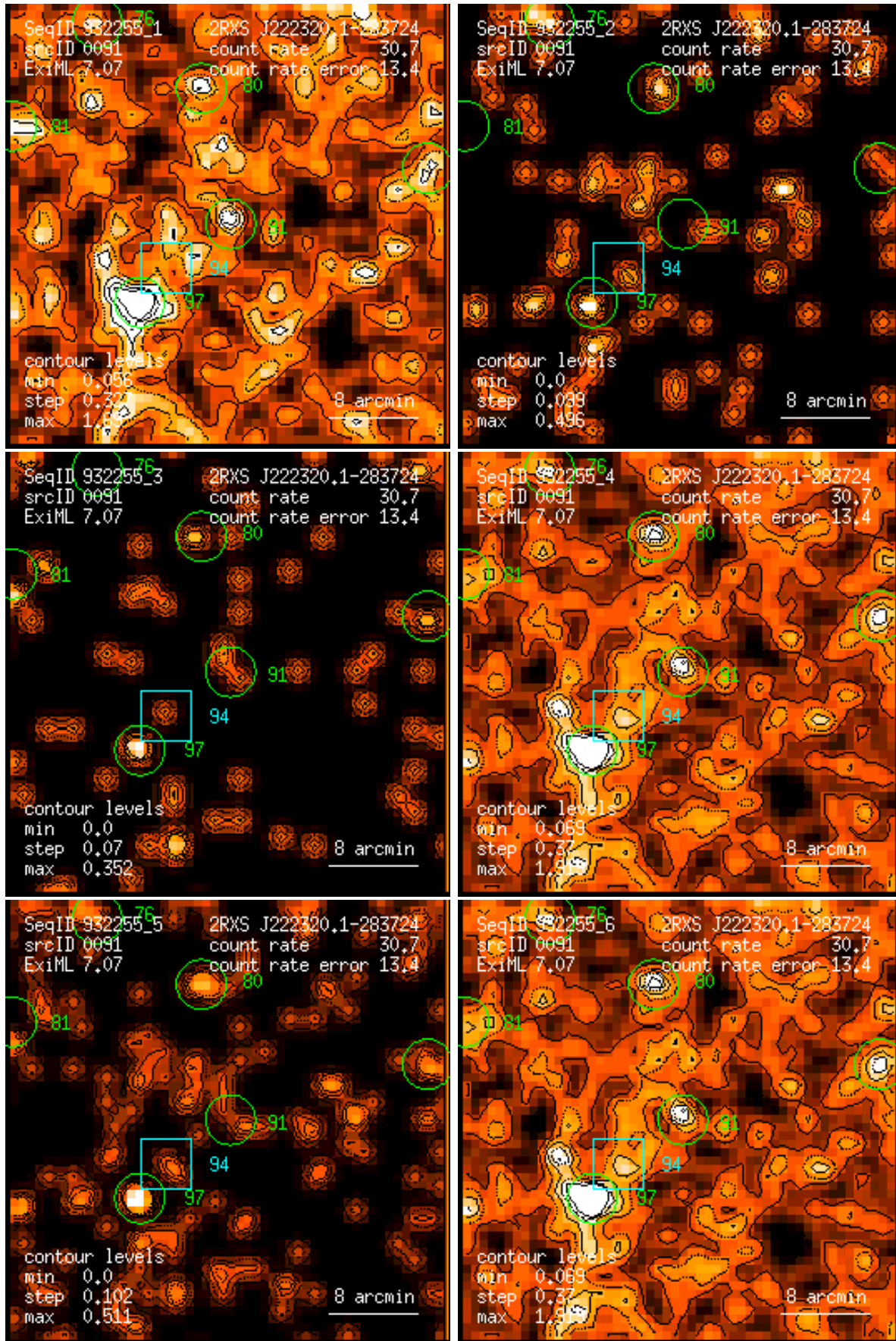
Figure 91: RASS 932255: detection 0091: band rate images, Gaussian filter: (1) PSPC channels 11 – 41, (2) 52 – 90, (3) 91 – 201, (4) 11 – 235, (5) 52 – 201, (6) 11 – 201. Broad band rates in counts/ks. Band rate contour levels in counts/ks/arcmin 2 .
