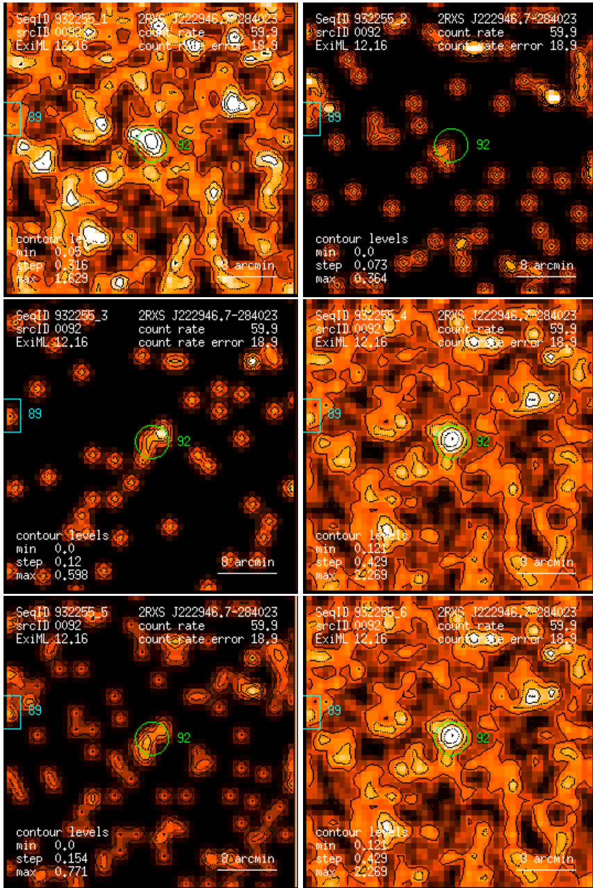
Figure 92: RASS 932255: detection 0092: band rate images, Gaussian filter: (1) PSPC channels 11 – 41, (2) 52 – 90, (3) 91 – 201, (4) 11 – 235, (5) 52 – 201, (6) 11 – 201. Broad band rates in counts/ks. Band rate contour levels in counts/ks/arcmin 2 .
