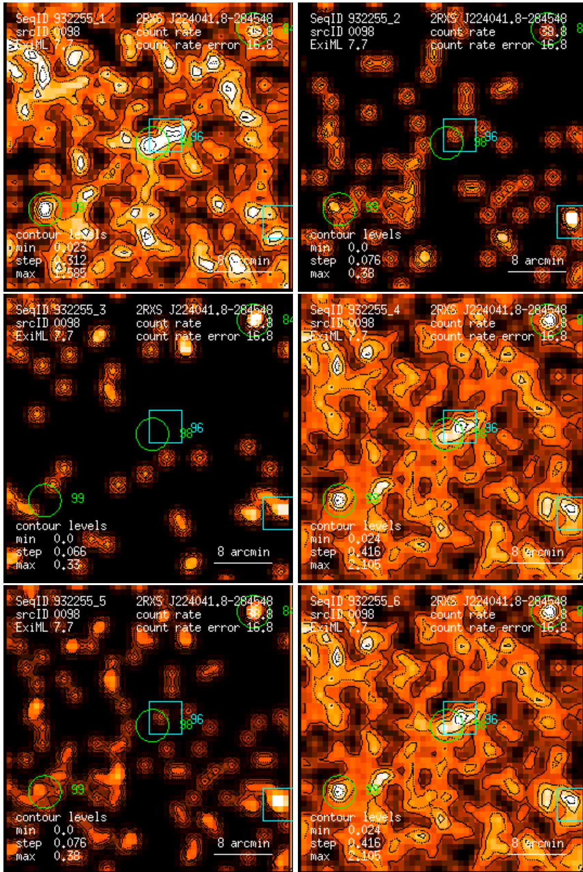
Figure 98: RASS 932255: detection 0098: band rate images, Gaussian filter: (1) PSPC channels 11 – 41, (2) 52 – 90, (3) 91 – 201, (4) 11 – 235, (5) 52 – 201, (6) 11 – 201. Broad band rates in counts/ks. Band rate contour levels in counts/ks/arcmin 2 .
