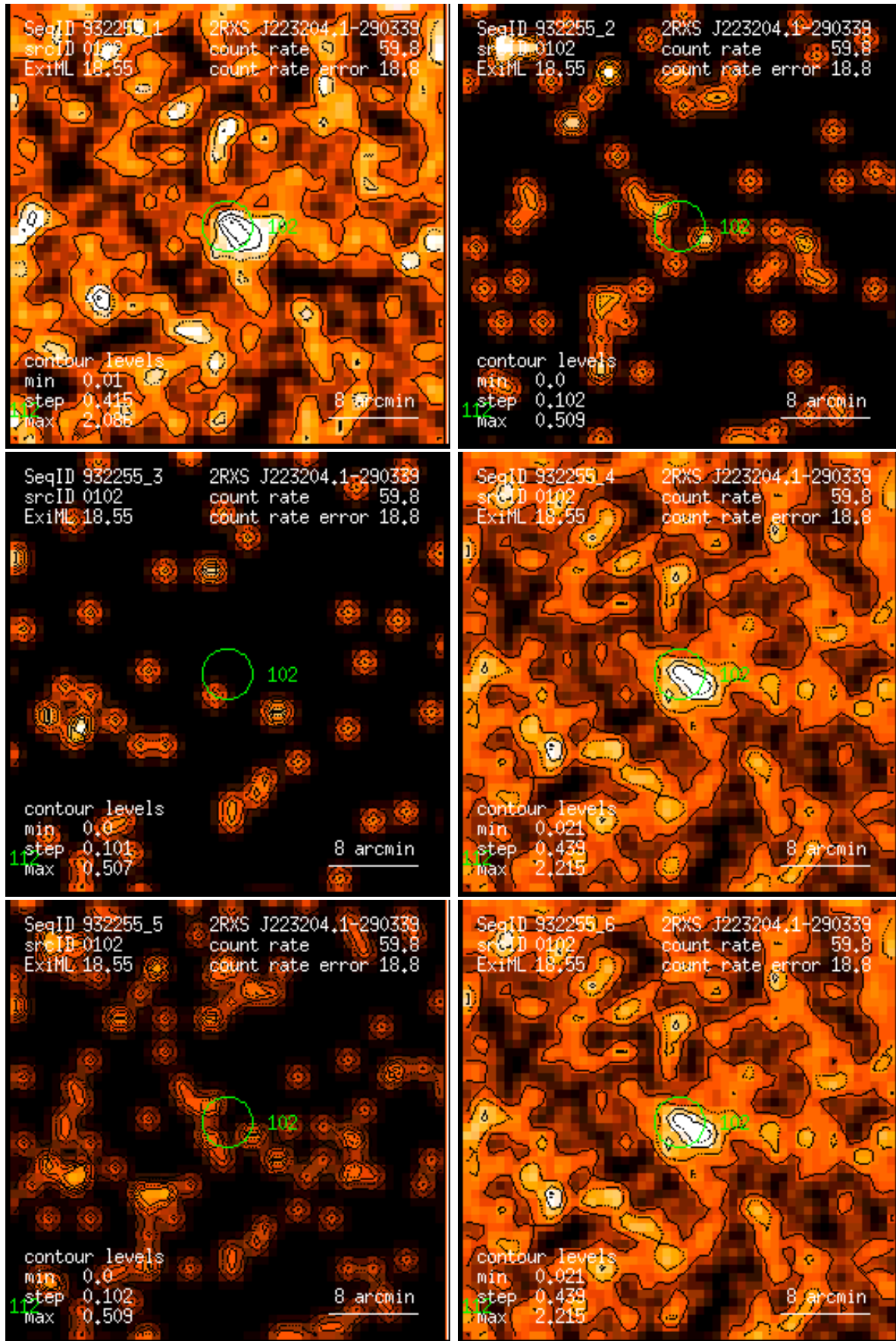
Figure 102: RASS 932255: detection 0102: band rate images, Gaussian filter: (1) PSPC channels 11 – 41, (2) 52 – 90, (3) 91 – 201, (4) 11 – 235, (5) 52 – 201, (6) 11 – 201. Broad band rates in counts/ks. Band rate contour levels in counts/ks/arcmin 2 .
