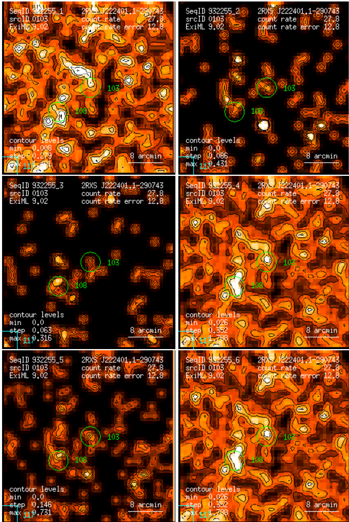
Figure 103: RASS 932255: detection 0103: band rate images, Gaussian filter: (1) PSPC channels 11 – 41, (2) 52 – 90, (3) 91 – 201, (4) 11 – 235, (5) 52 – 201, (6) 11 – 201. Broad band rates in counts/ks. Band rate contour levels in counts/ks/arcmin 2 .
