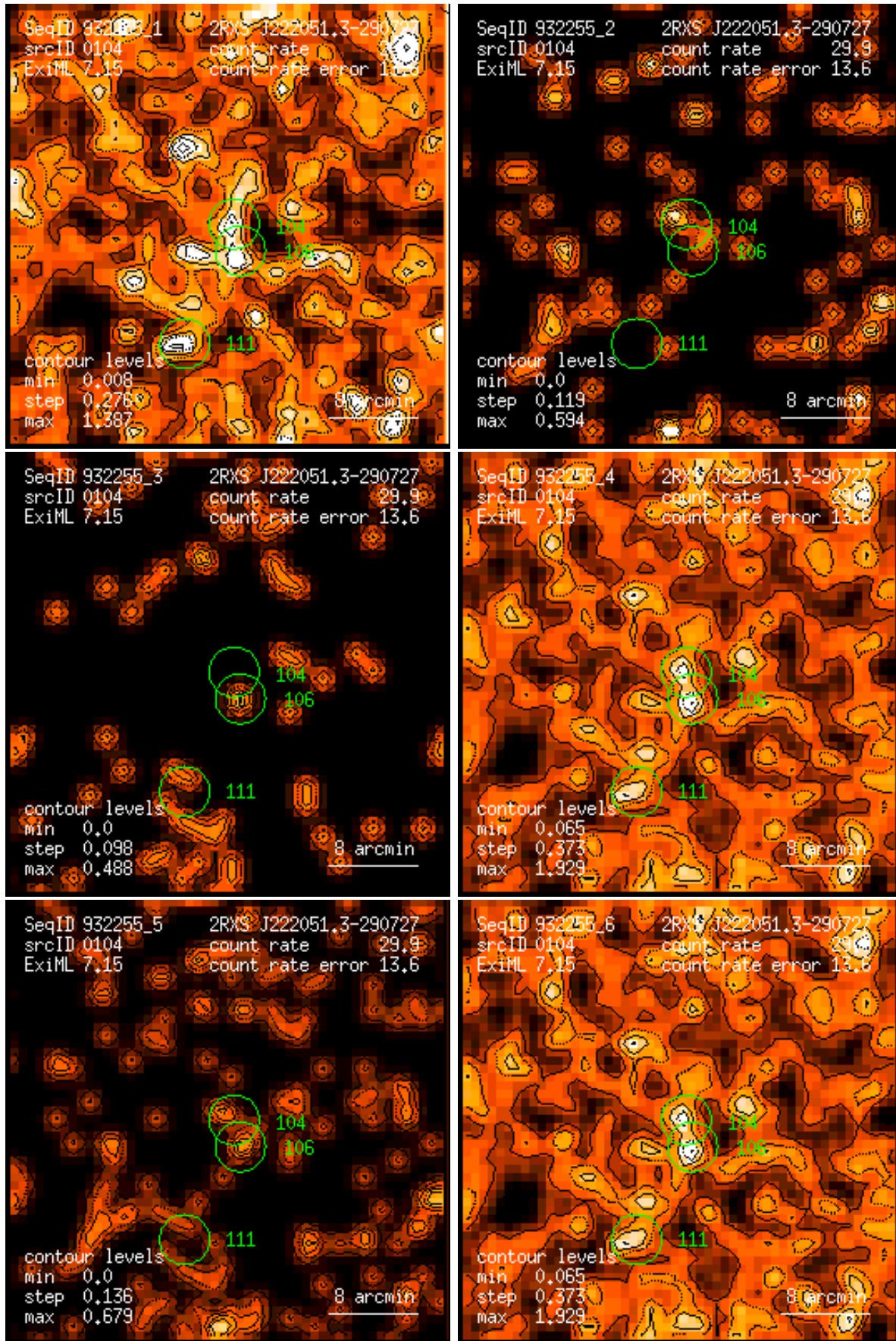
Figure 104: RASS 932255: detection 0104: band rate images, Gaussian filter: (1) PSPC channels 11 – 41, (2) 52 – 90, (3) 91 – 201, (4) 11 – 235, (5) 52 – 201, (6) 11 – 201. Broad band rates in counts/ks. Band rate contour levels in counts/ks/arcmin 2 .
