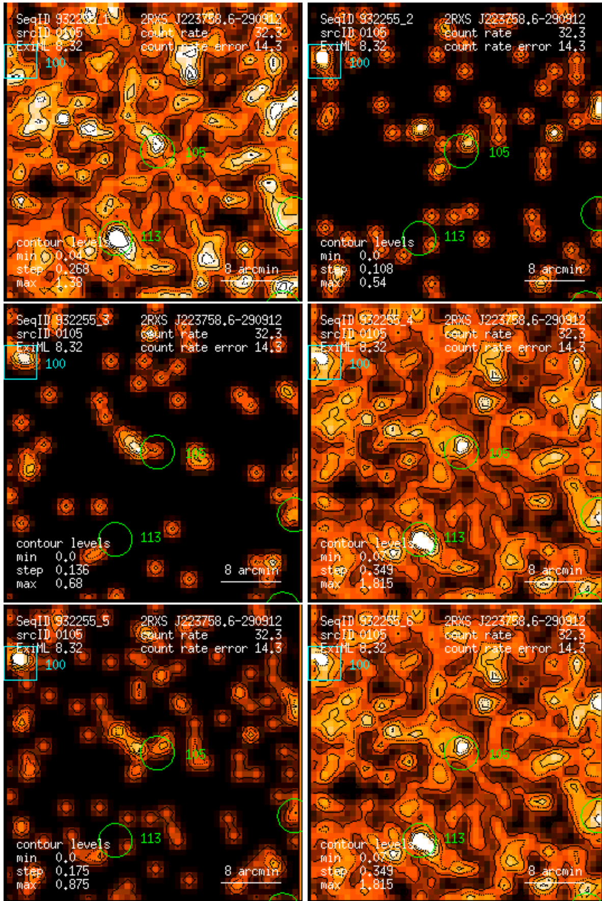
Figure 105: RASS 932255: detection 0105: band rate images, Gaussian filter: (1) PSPC channels 11 – 41, (2) 52 – 90, (3) 91 – 201, (4) 11 – 235, (5) 52 – 201, (6) 11 – 201. Broad band rates in counts/ks. Band rate contour levels in counts/ks/arcmin 2 .
