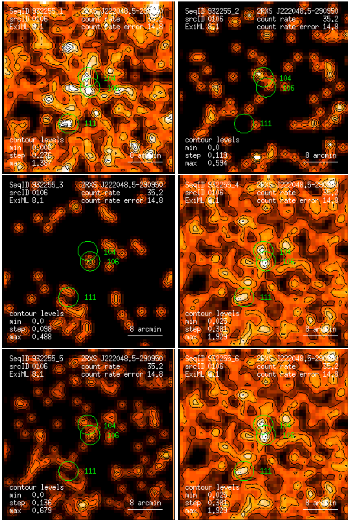
Figure 106: RASS 932255: detection 0106: band rate images, Gaussian filter: (1) PSPC channels 11 – 41, (2) 52 – 90, (3) 91 – 201, (4) 11 – 235, (5) 52 – 201, (6) 11 – 201. Broad band rates in counts/ks. Band rate contour levels in counts/ks/arcmin 2 .
