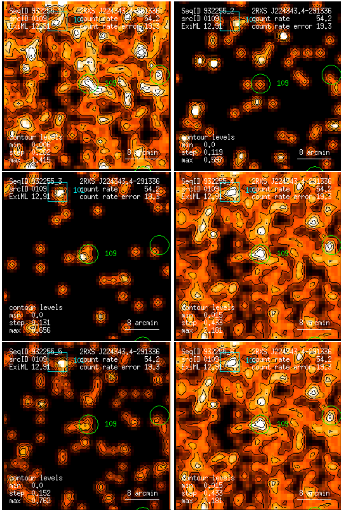
Figure 109: RASS 932255: detection 0109: band rate images, Gaussian filter: (1) PSPC channels 11 – 41, (2) 52 – 90, (3) 91 – 201, (4) 11 – 235, (5) 52 – 201, (6) 11 – 201. Broad band rates in counts/ks. Band rate contour levels in counts/ks/arcmin 2 .
