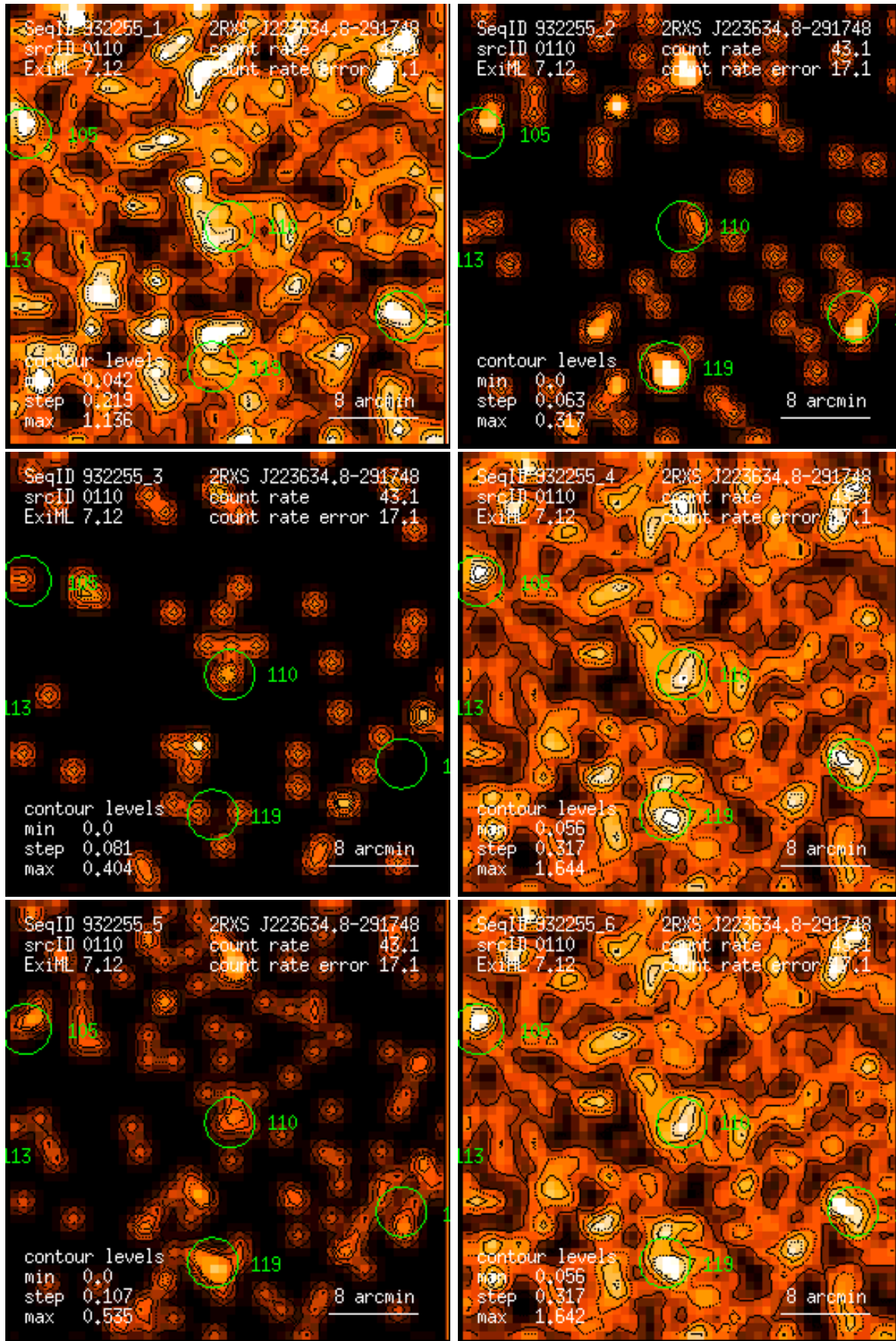
Figure 110: RASS 932255: detection 0110: band rate images, Gaussian filter: (1) PSPC channels 11 – 41, (2) 52 – 90, (3) 91 – 201, (4) 11 – 235, (5) 52 – 201, (6) 11 – 201. Broad band rates in counts/ks. Band rate contour levels in counts/ks/arcmin 2 .
