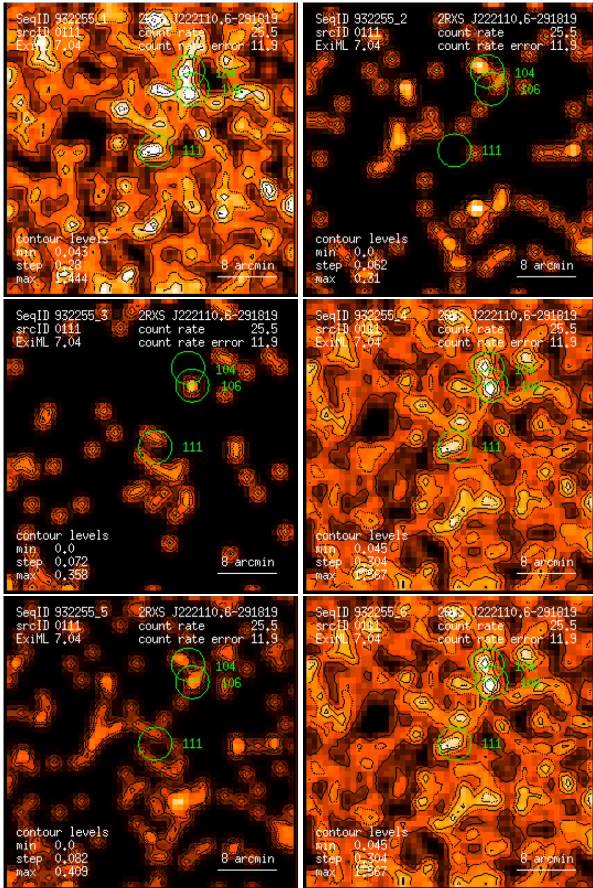
Figure 111: RASS 932255: detection 0111: band rate images, Gaussian filter: (1) PSPC channels 11 – 41, (2) 52 – 90, (3) 91 – 201, (4) 11 – 235, (5) 52 – 201, (6) 11 – 201. Broad band rates in counts/ks. Band rate contour levels in counts/ks/arcmin 2 .
