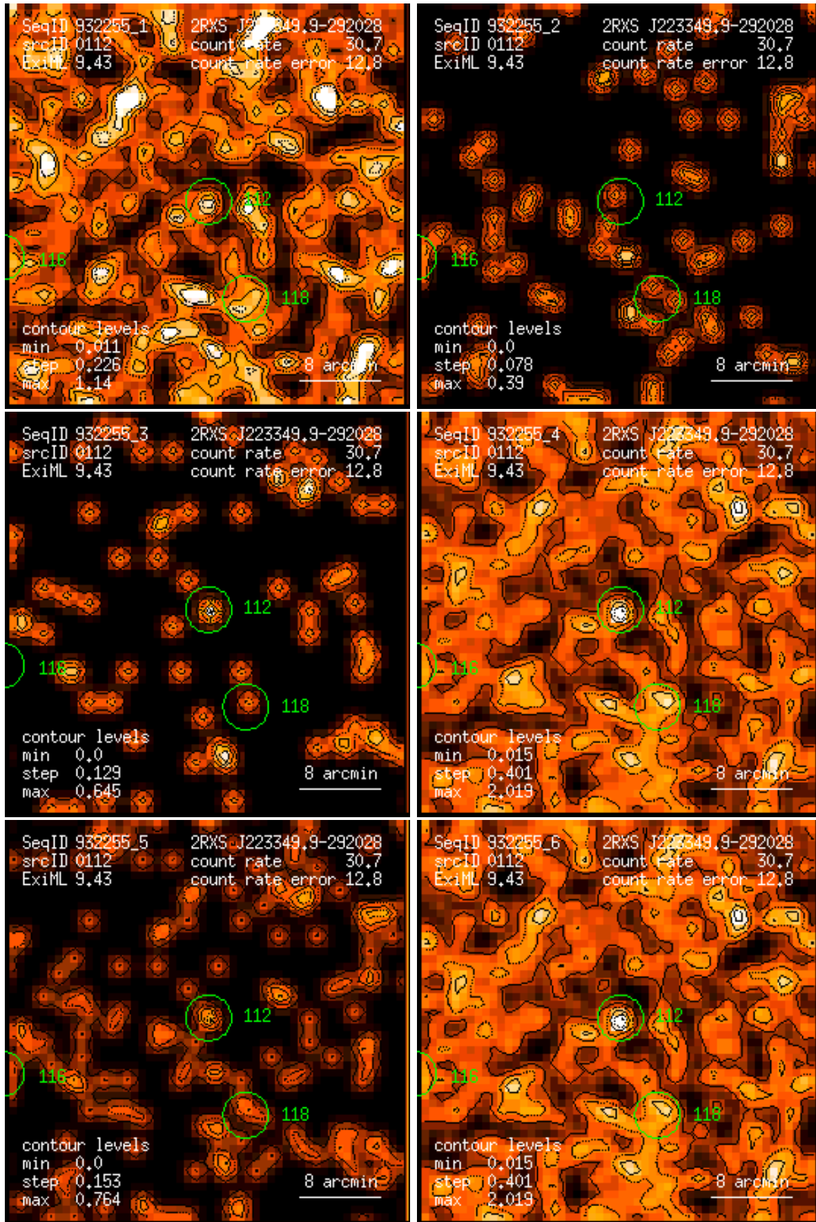
Figure 112: RASS 932255: detection 0112: band rate images, Gaussian filter: (1) PSPC channels 11 – 41, (2) 52 – 90, (3) 91 – 201, (4) 11 – 235, (5) 52 – 201, (6) 11 – 201. Broad band rates in counts/ks. Band rate contour levels in counts/ks/arcmin 2 .
