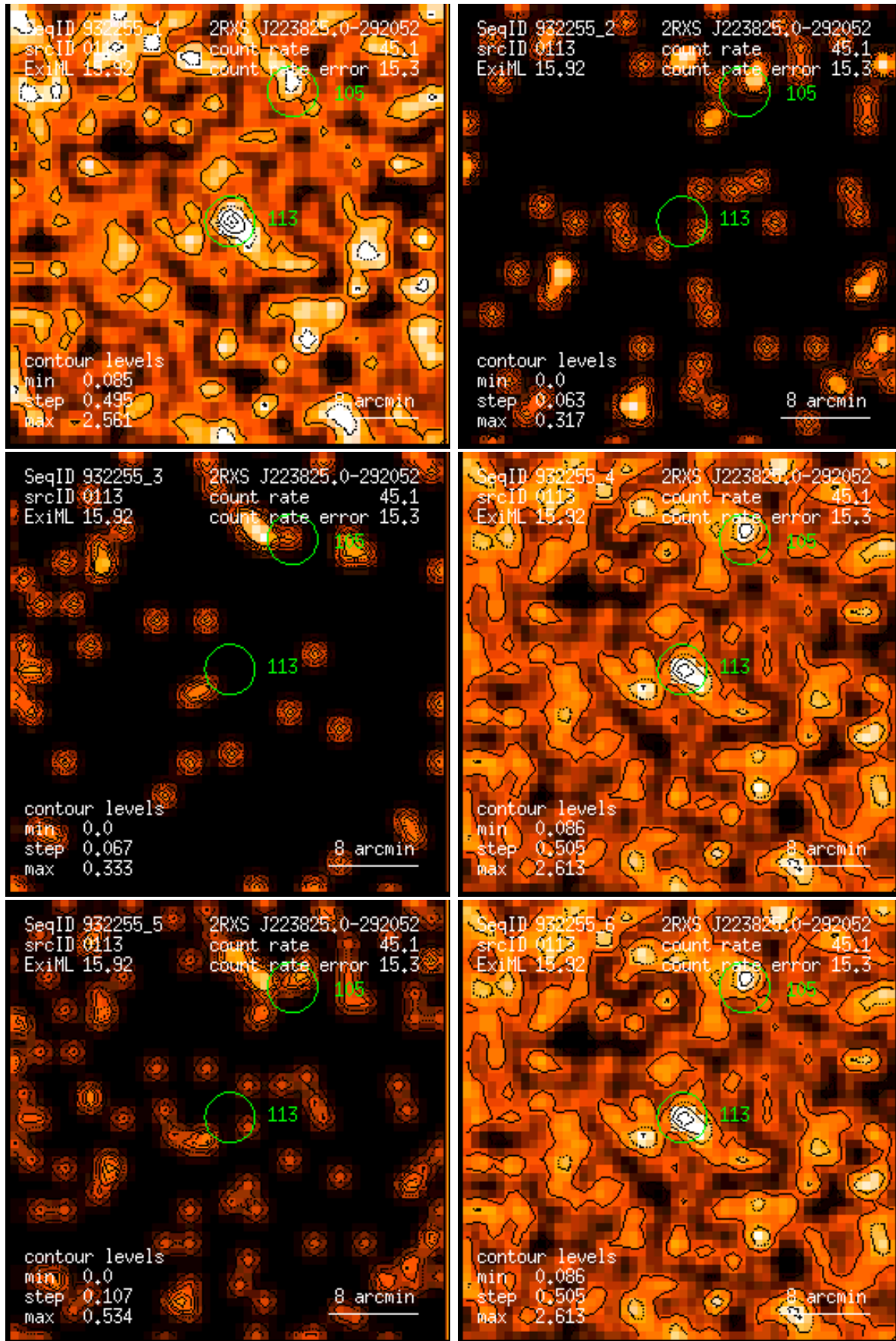
Figure 113: RASS 932255: detection 0113: band rate images, Gaussian filter: (1) PSPC channels 11 – 41, (2) 52 – 90, (3) 91 – 201, (4) 11 – 235, (5) 52 – 201, (6) 11 – 201. Broad band rates in counts/ks. Band rate contour levels in counts/ks/arcmin 2 .
