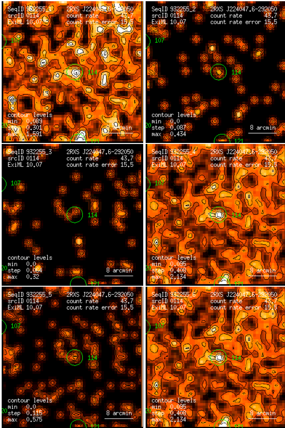
Figure 114: RASS 932255: detection 0114: band rate images, Gaussian filter: (1) PSPC channels 11 – 41, (2) 52 – 90, (3) 91 – 201, (4) 11 – 235, (5) 52 – 201, (6) 11 – 201. Broad band rates in counts/ks. Band rate contour levels in counts/ks/arcmin 2 .
