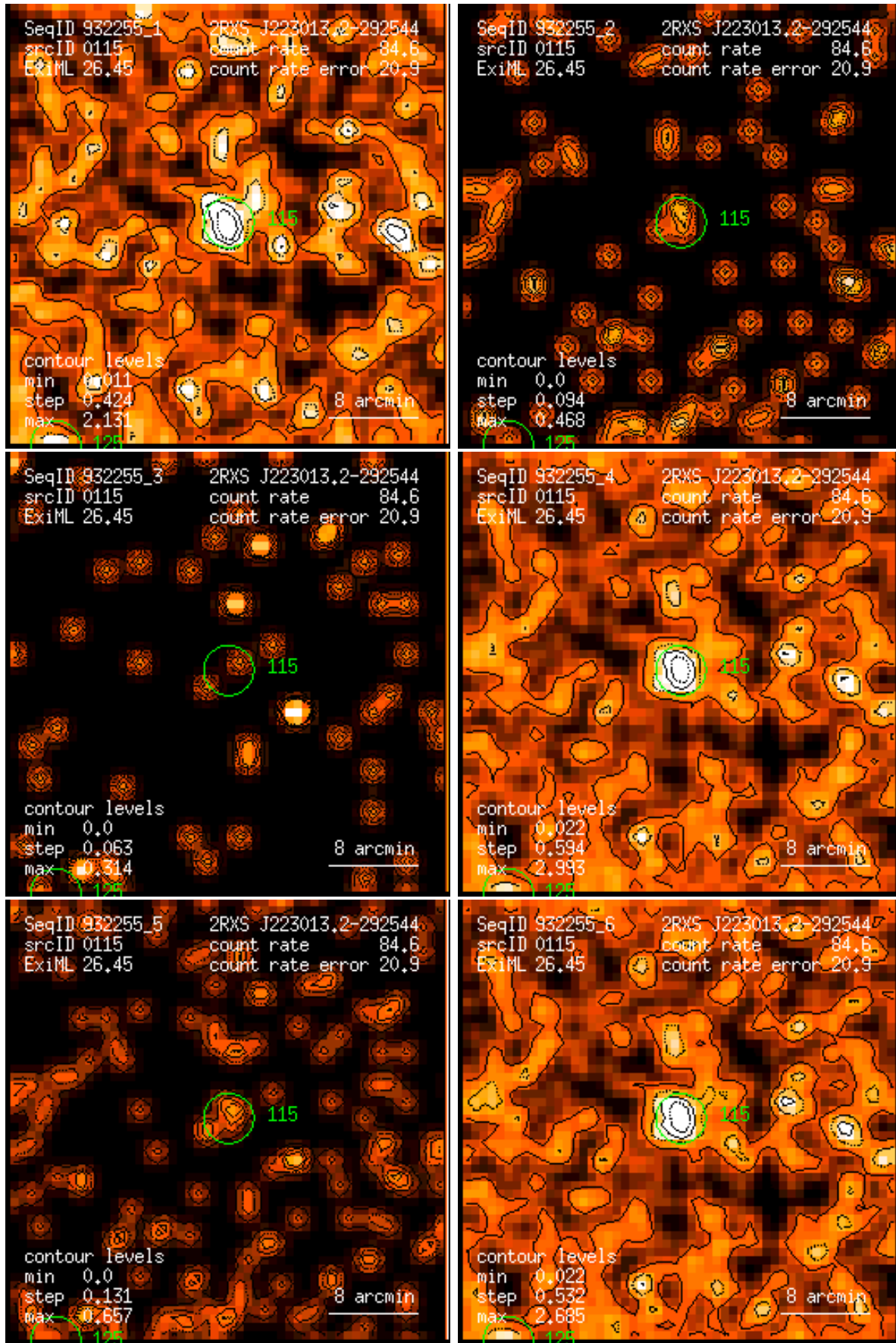
Figure 115: RASS 932255: detection 0115: band rate images, Gaussian filter: (1) PSPC channels 11 – 41, (2) 52 – 90, (3) 91 – 201, (4) 11 – 235, (5) 52 – 201, (6) 11 – 201. Broad band rates in counts/ks. Band rate contour levels in counts/ks/arcmin 2 .
