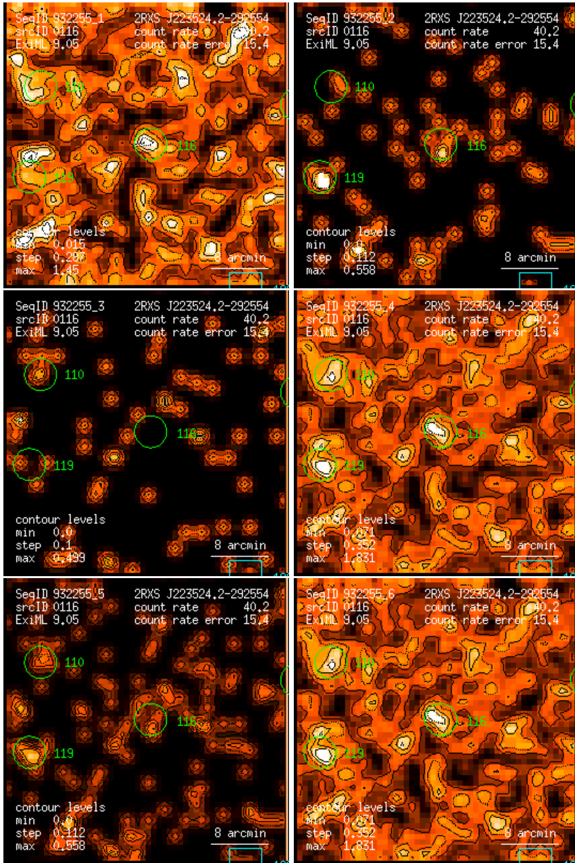
Figure 116: RASS 932255: detection 0116: band rate images, Gaussian filter: (1) PSPC channels 11 – 41, (2) 52 – 90, (3) 91 – 201, (4) 11 – 235, (5) 52 – 201, (6) 11 – 201. Broad band rates in counts/ks. Band rate contour levels in counts/ks/arcmin 2 .
