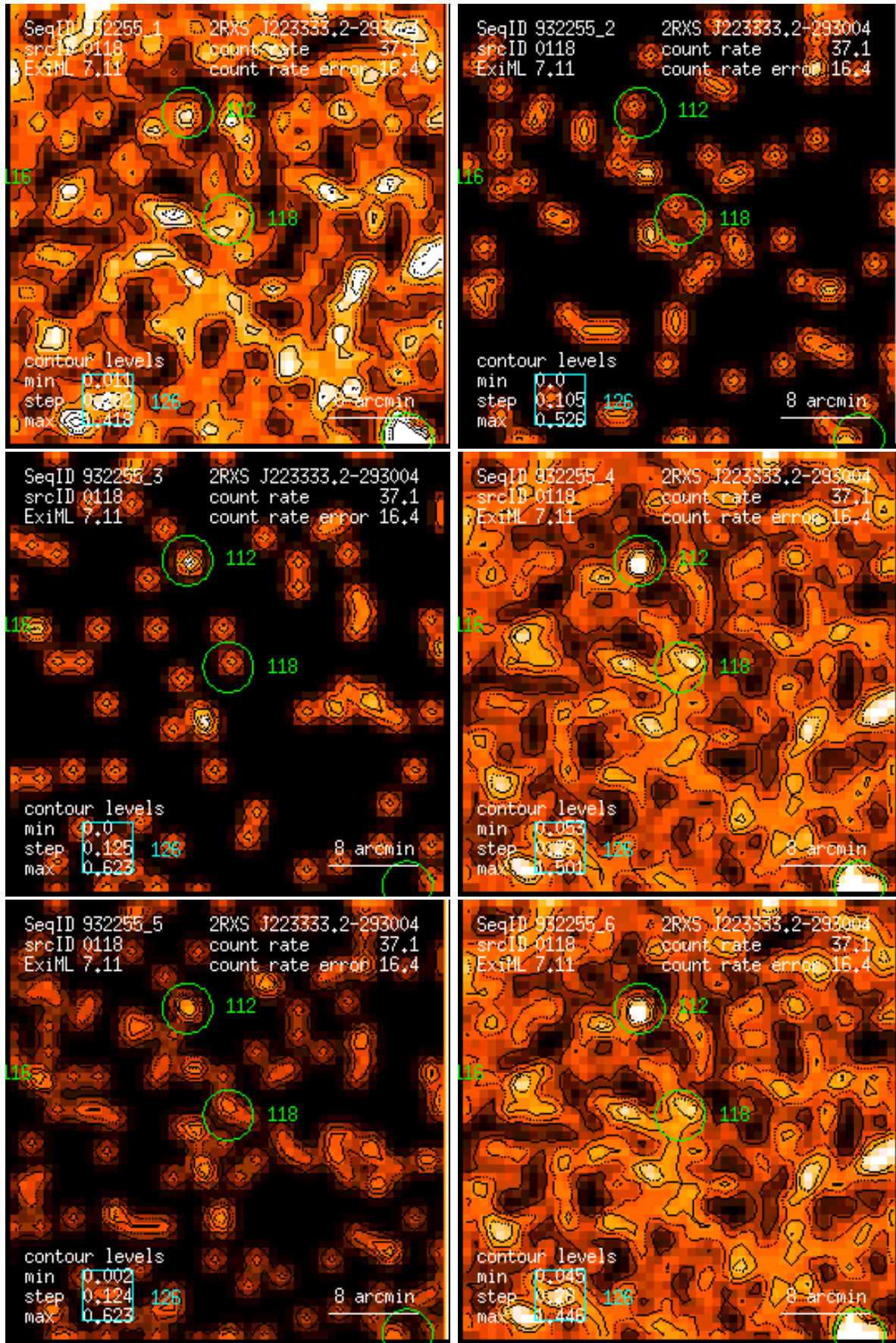
Figure 118: RASS 932255: detection 0118: band rate images, Gaussian filter: (1) PSPC channels 11 – 41, (2) 52 – 90, (3) 91 – 201, (4) 11 – 235, (5) 52 – 201, (6) 11 – 201. Broad band rates in counts/ks. Band rate contour levels in counts/ks/arcmin 2 .
