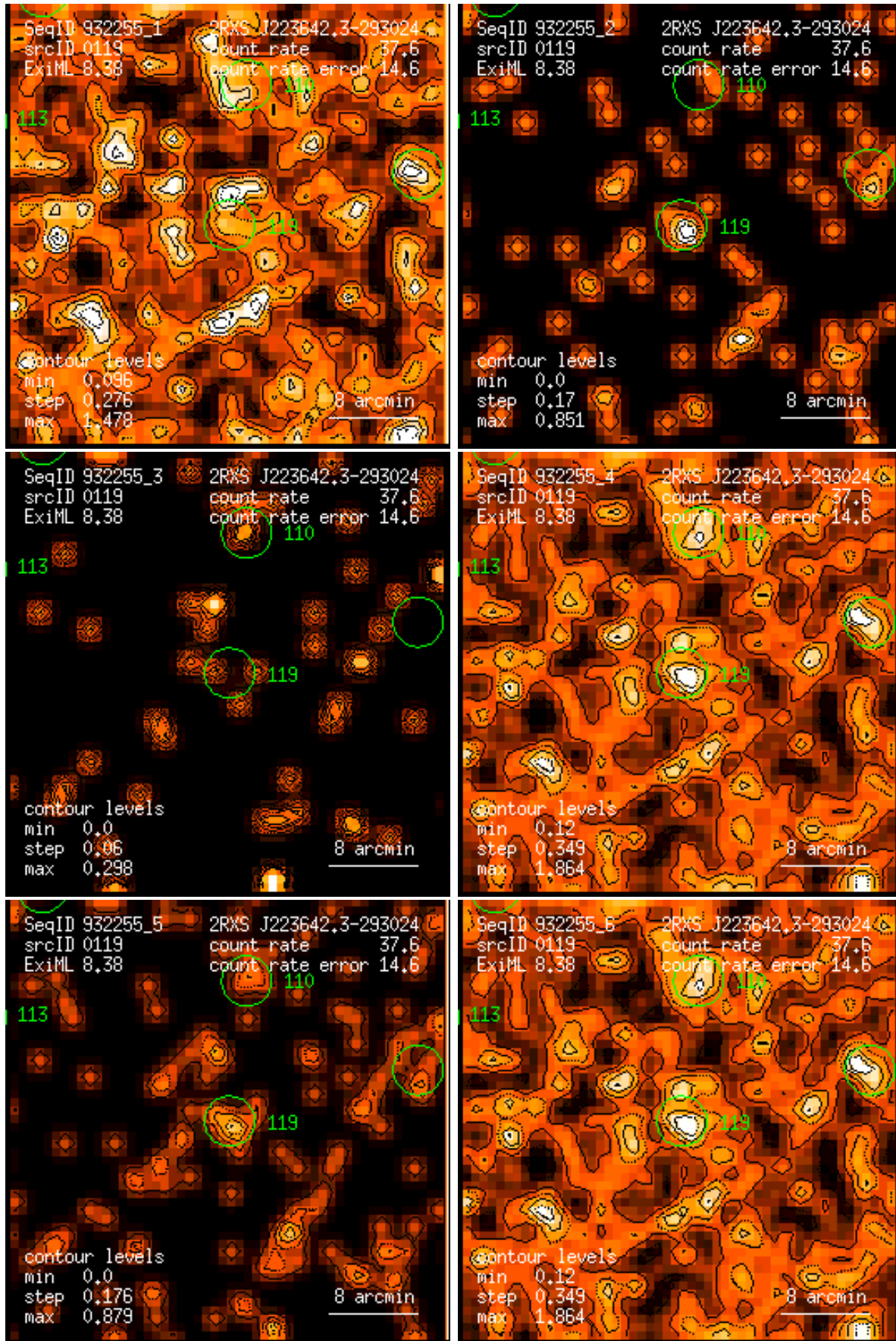
Figure 119: RASS 932255: detection 0119: band rate images, Gaussian filter: (1) PSPC channels 11 – 41, (2) 52 – 90, (3) 91 – 201, (4) 11 – 235, (5) 52 – 201, (6) 11 – 201. Broad band rates in counts/ks. Band rate contour levels in counts/ks/arcmin 2 .
