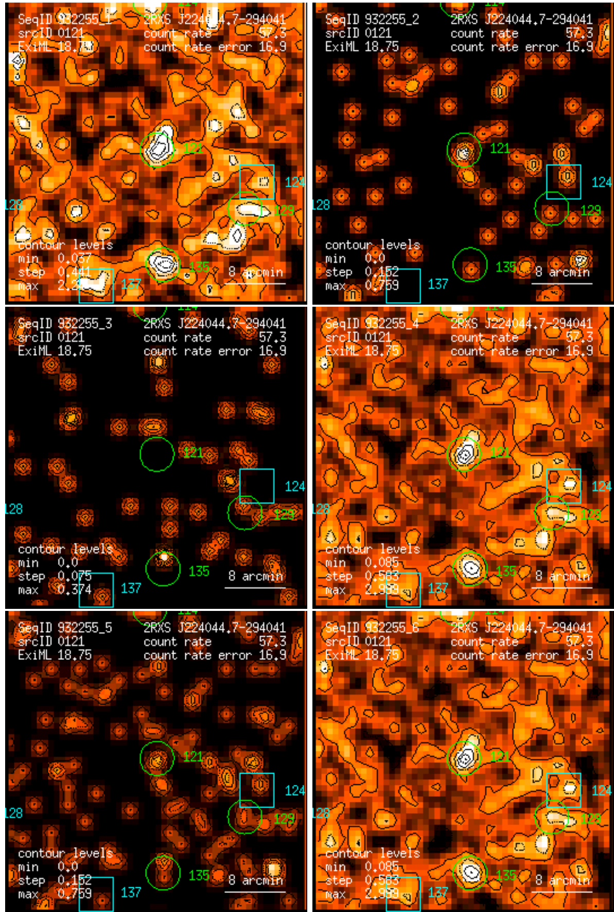
Figure 121: RASS 932255: detection 0121: band rate images, Gaussian filter: (1) PSPC channels 11 – 41, (2) 52 – 90, (3) 91 – 201, (4) 11 – 235, (5) 52 – 201, (6) 11 – 201. Broad band rates in counts/ks. Band rate contour levels in counts/ks/arcmin 2 .
