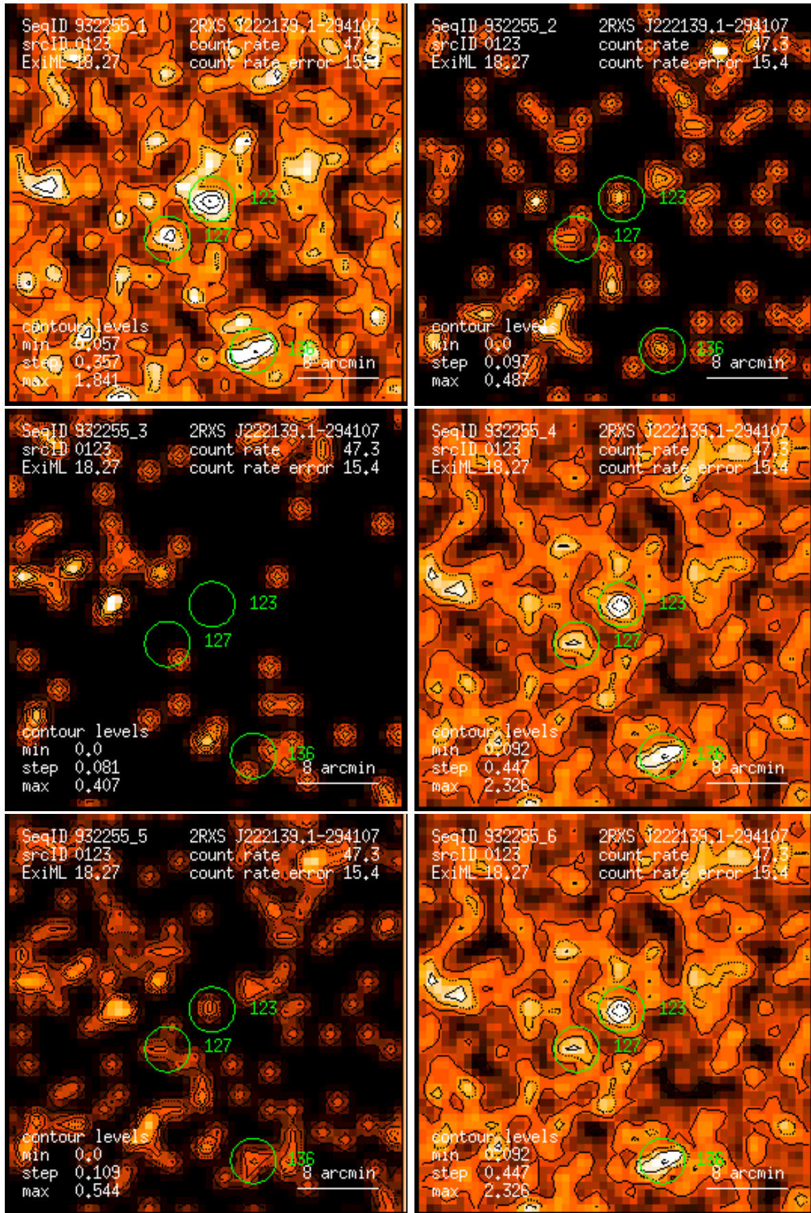
Figure 123: RASS 932255: detection 0123: band rate images, Gaussian filter: (1) PSPC channels 11 – 41, (2) 52 – 90, (3) 91 – 201, (4) 11 – 235, (5) 52 – 201, (6) 11 – 201. Broad band rates in counts/ks. Band rate contour levels in counts/ks/arcmin 2 .
