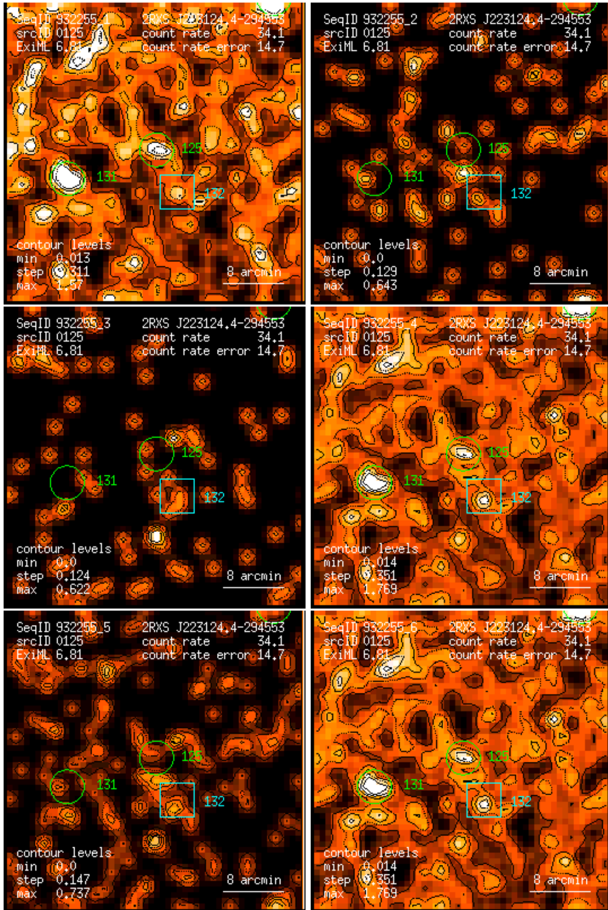
Figure 125: RASS 932255: detection 0125: band rate images, Gaussian filter: (1) PSPC channels 11 – 41, (2) 52 – 90, (3) 91 – 201, (4) 11 – 235, (5) 52 – 201, (6) 11 – 201. Broad band rates in counts/ks. Band rate contour levels in counts/ks/arcmin 2 .
